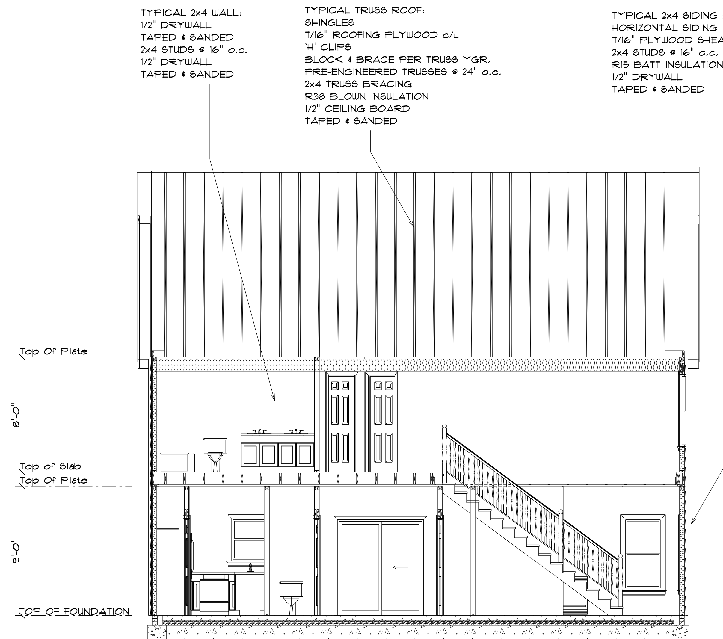
SECTION THROUGH SCALE: 1" = 1/4"
