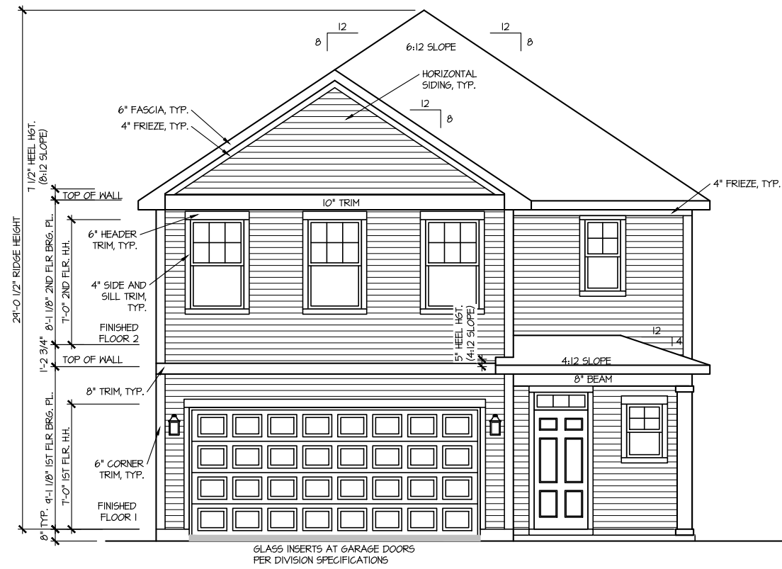
FRONT ELEVATION I
