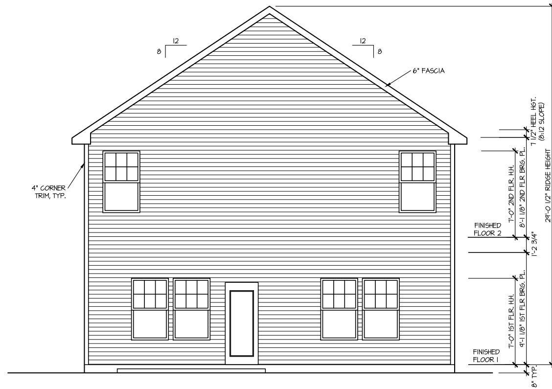
REAR ELEVATION I
