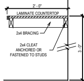
COUNTERTOP DETAIL SCALE: 1/2" = 1'-0"
