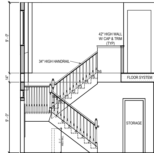
STAIR SECTION
