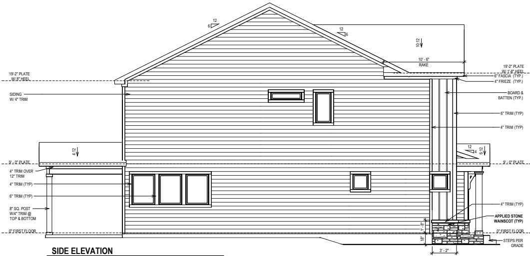
SIDE ELEVATION
