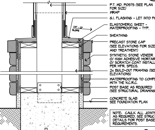
COLUMN BASE W/ STONE SCALE 1/2"=1'-0" SE-04068a
