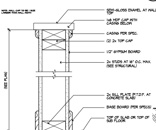
PONY WALL SCALE 3/4"=1'-0" SE-04072a
