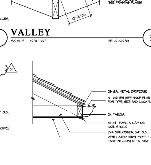
TYPICAL EAVE GUTTER
