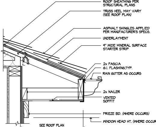
EAVE
