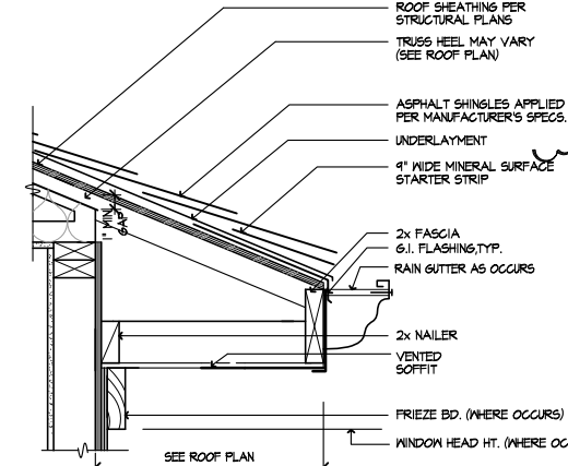
EAVE
