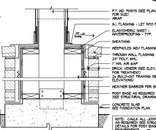
COLUMN BASE W/ BRICK SCALE 1/2"=1'-0" SE-04064a
