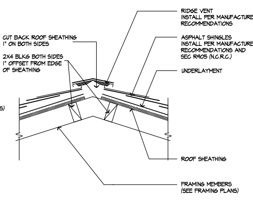
RIDGE VENT
