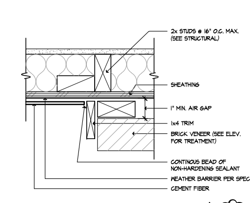
SIDING TO BRICK SCALE 3/4"=1'-0" SE-04070a
