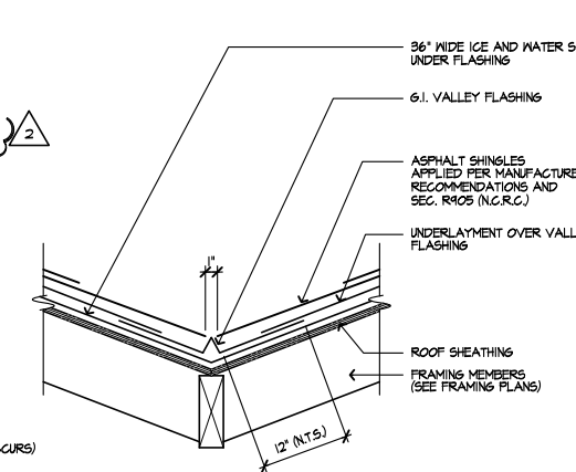
VALLEY
