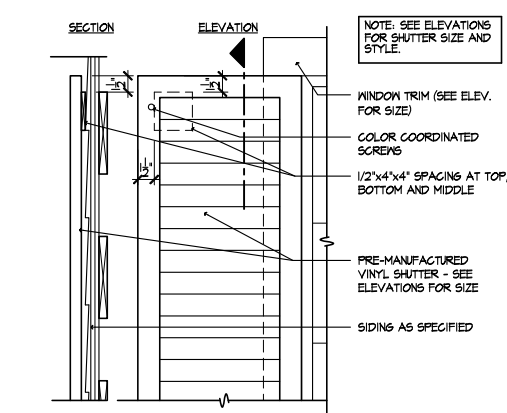
WINDOW SHUTTER SCALE 1/2"=1'-0" SE-04062a
