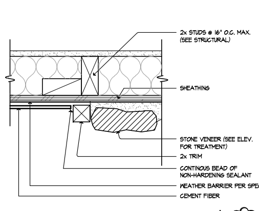
SIDING TO STONE SCALE 3/4"=1'-0" SE-04066a
