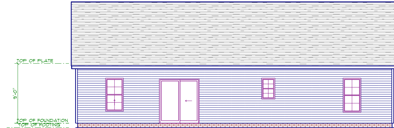
REAR ELEVATION
