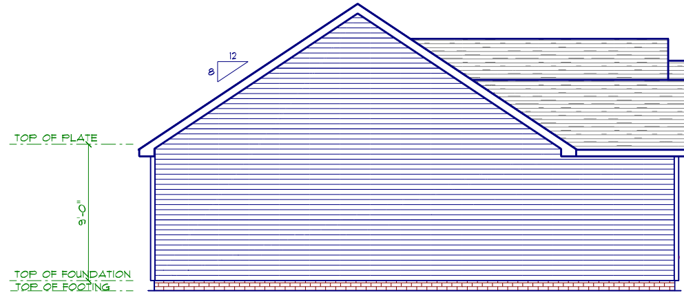
LEFT ELEVATION
