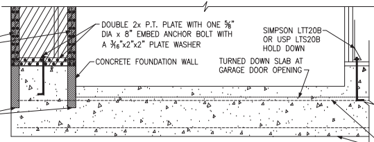
(C) METHOD CS-EPF: ENGINEERED PORTAL FRAME WITH HOLD-DOWNS
