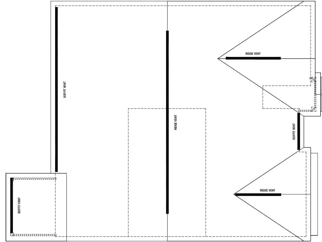
ROOF PLAN VENT CALCS.
