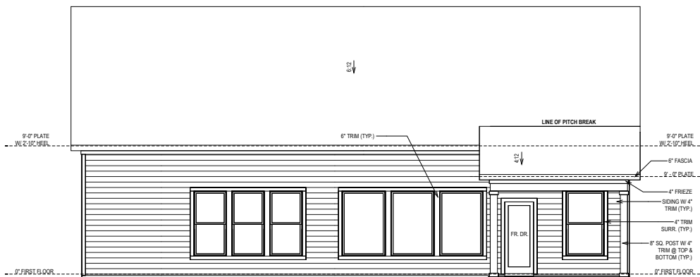
REAR ELEVATION
