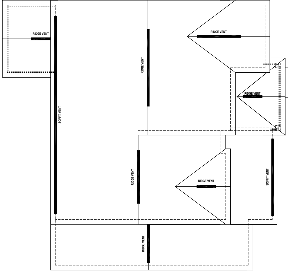
ROOF PLAN W/ CALCS
