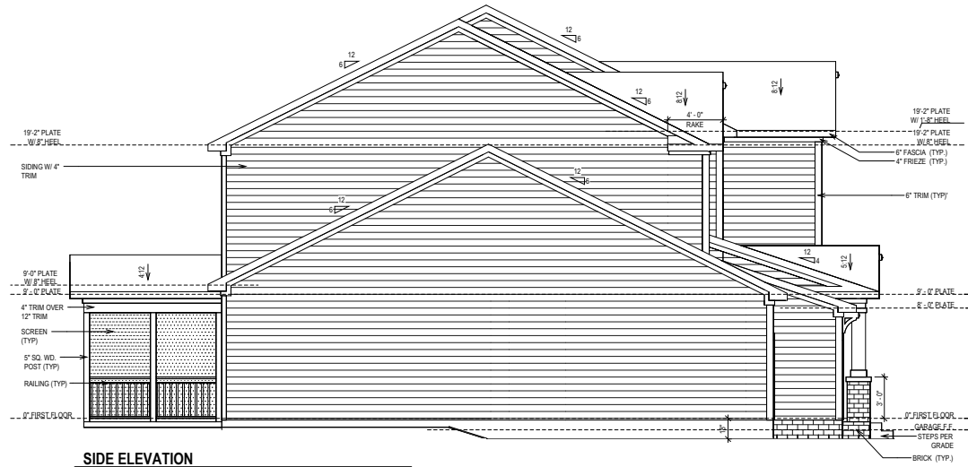
SIDE ELEVATION
