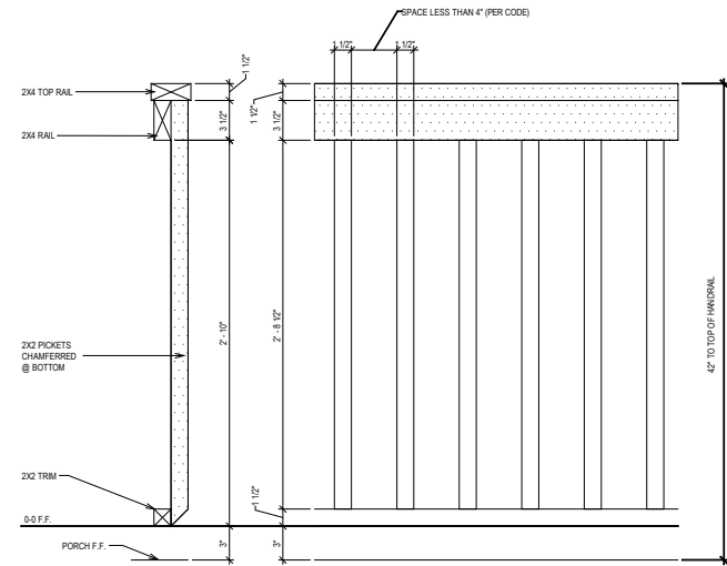
42" PORCH RAIL DETAIL
