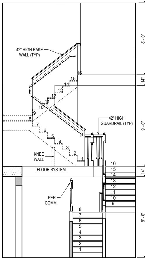
STAIR SECTION
