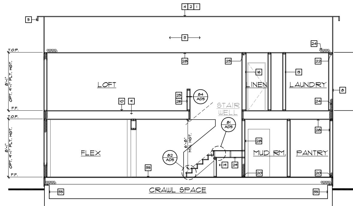
SECTION "C"
