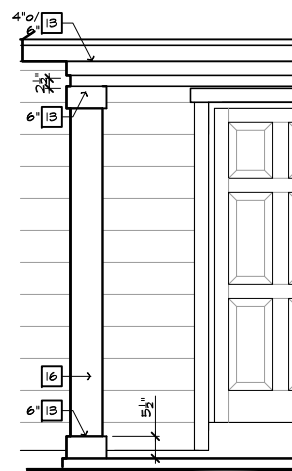
DETAIL 'B'
