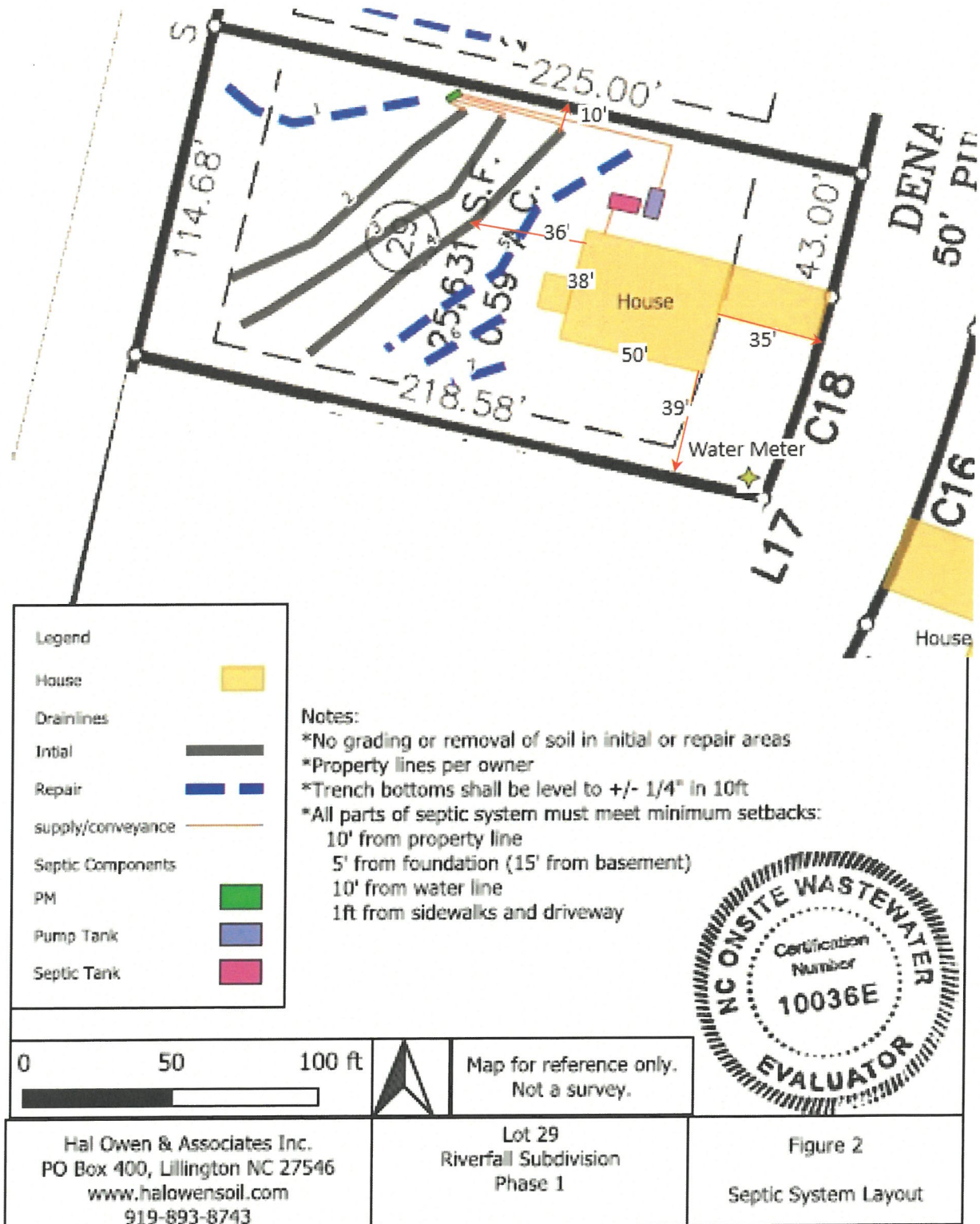
Figure 1. As-built Septic System Installation
