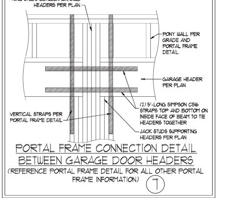
PORTAL FRAME CONNECTION DETAIL BETWEEN GARAGE DOOR HEADERS (REFERENCE PORTAL FRAME DETAIL FOR ALL OTHER PORTAL FRAME INFORMATION) ⑦
