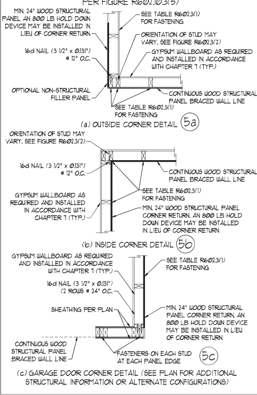
(a) OUTSIDE CORNER DETAIL (b) INSIDE CORNER DETAIL
