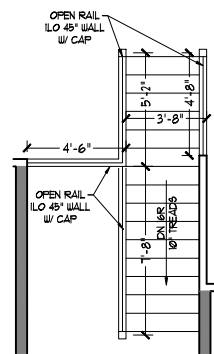
OPTIONAL OPEN RAIL ILO 45" WALL W/ CAP
