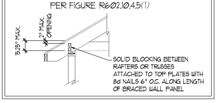
BRACED WALL PANEL CONNECTION TO PERPENDICULAR RAFTERS PER FIGURE R602.10.4.5(1)
