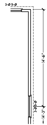
OPTIONAL WINDOW AT OWNER'S BEDROOM
