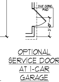
OPTIONAL 1-CAR GARAGE (NOT AVAILABLE W/ SIDE-LOAD GARAGE)
