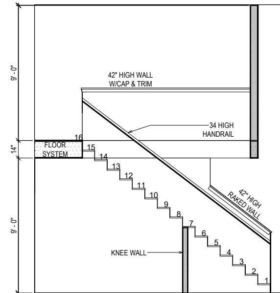
STAIR SECTION
