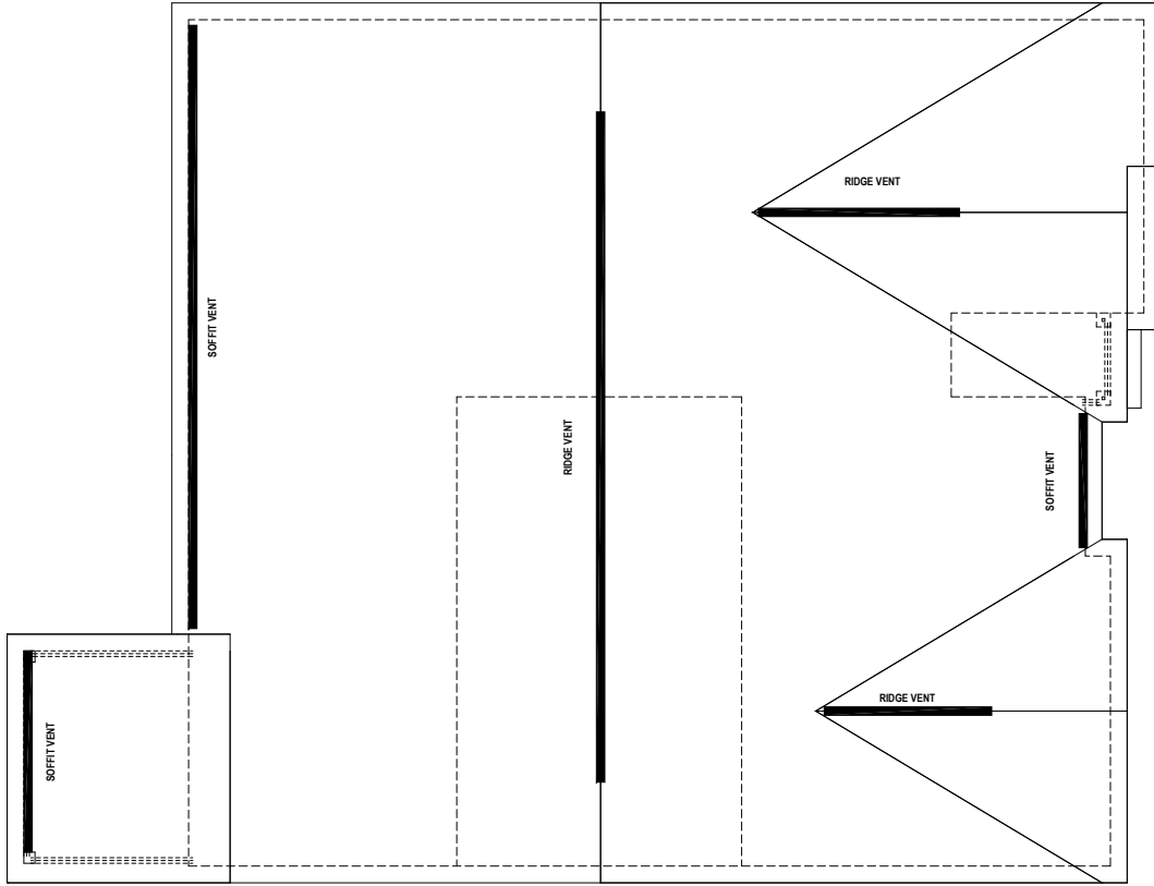
ROOF PLAN
