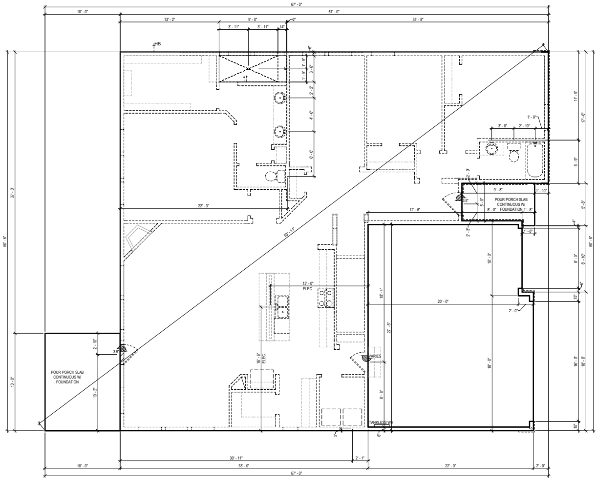
FIRST FLOOR
