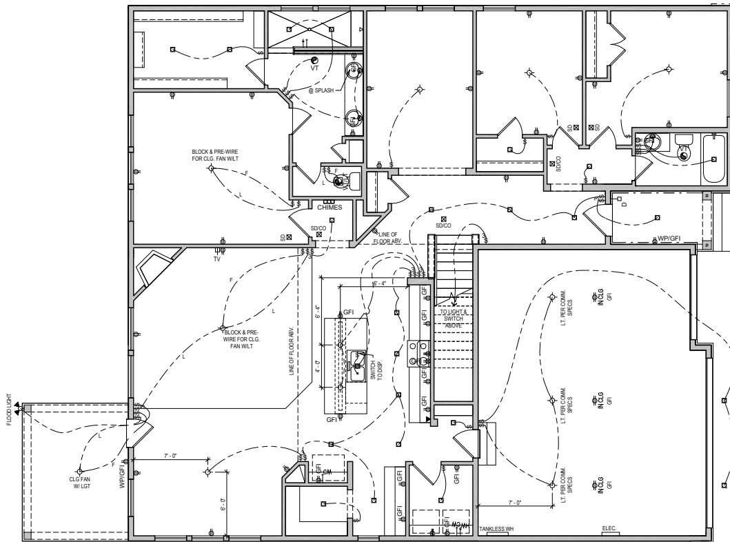
FIRST FLOOR
