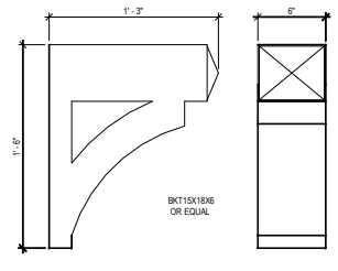
BRACKET DETAIL
