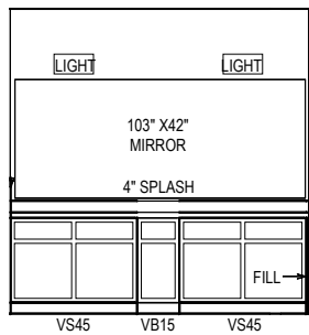
OWNER'S BATH
