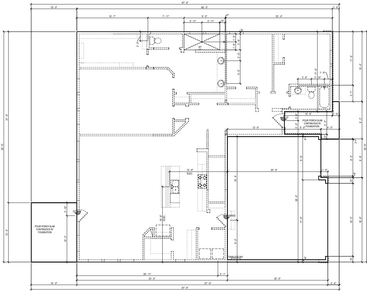
FIRST FLOOR
