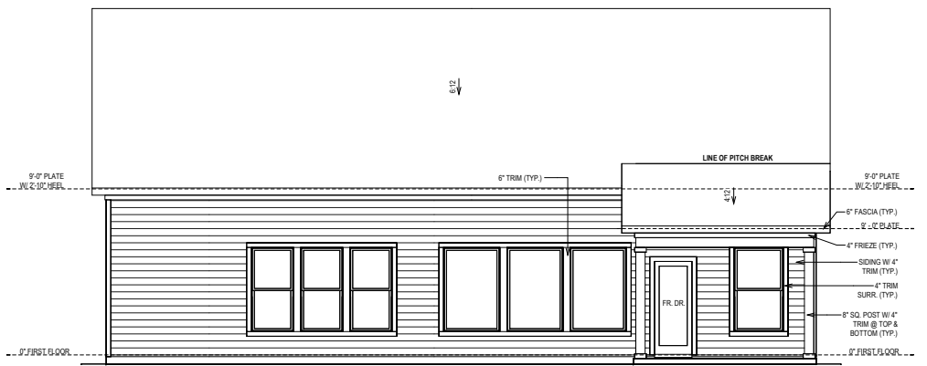
REAR ELEVATION
