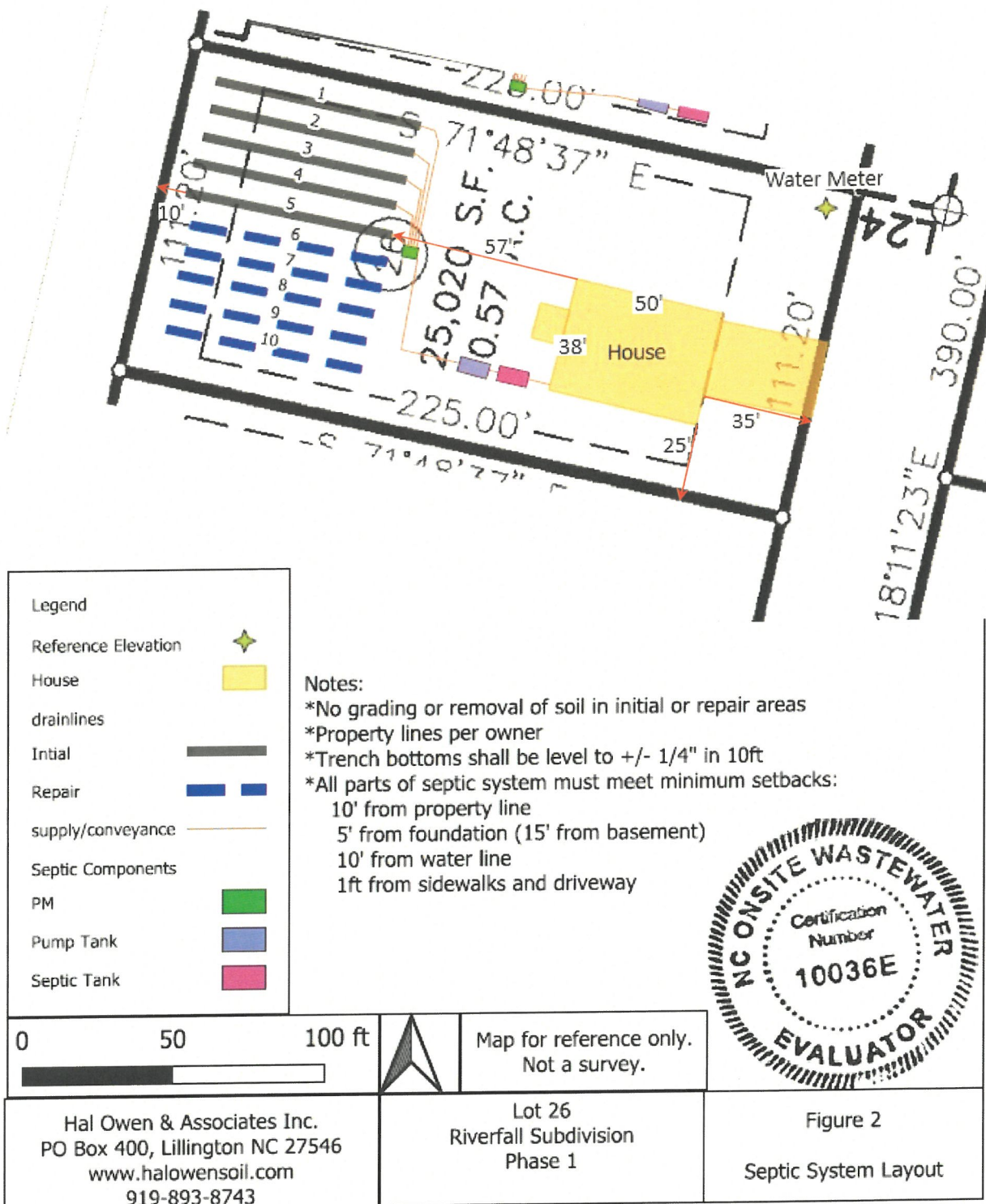
Figure 1. As-built Septic System Installation
