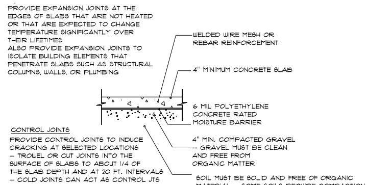
CONCRETE SLAB DETAILS / NOTES not to scale
