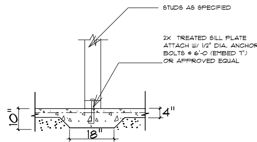
TYPICAL THICKENED SLAB not to scale
