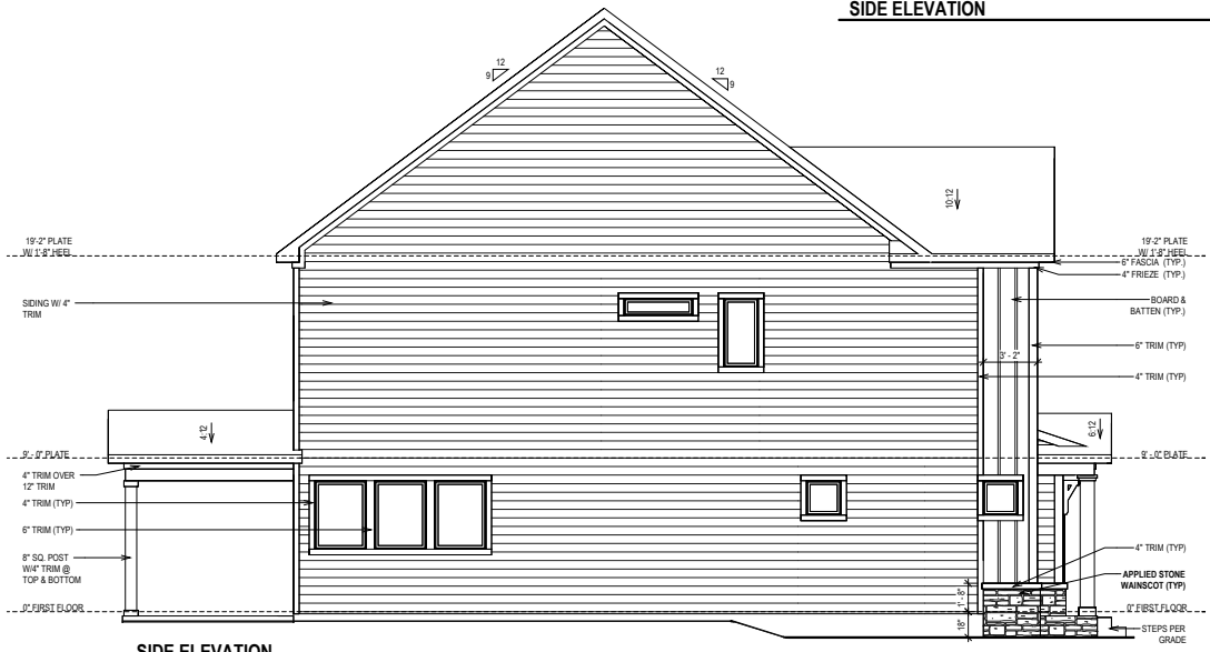
SIDE ELEVATION
