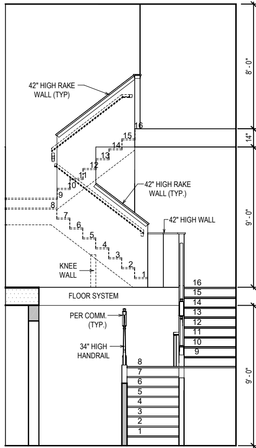
STAIR SECTION
