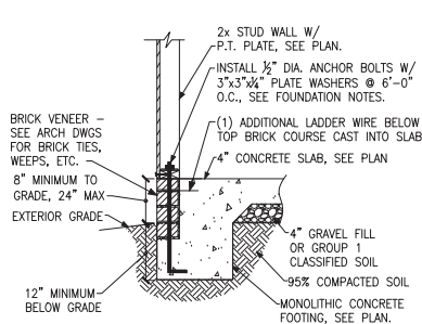
L FOUNDATION SECTION ALTERNATE EXTERIOR WALL
