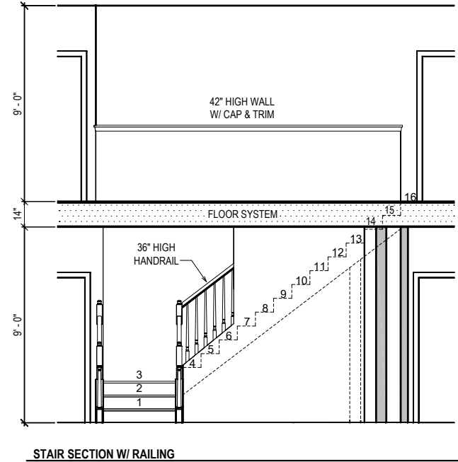
STAIR SECTION W/ RAILING
