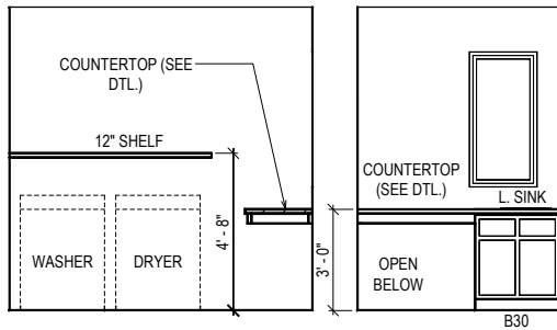
COUNTERTOP @ UTIL
