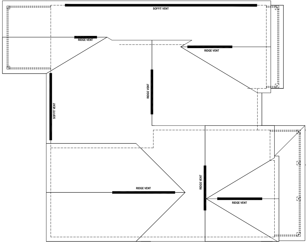
ROOF PLAN VENT CALCS.
