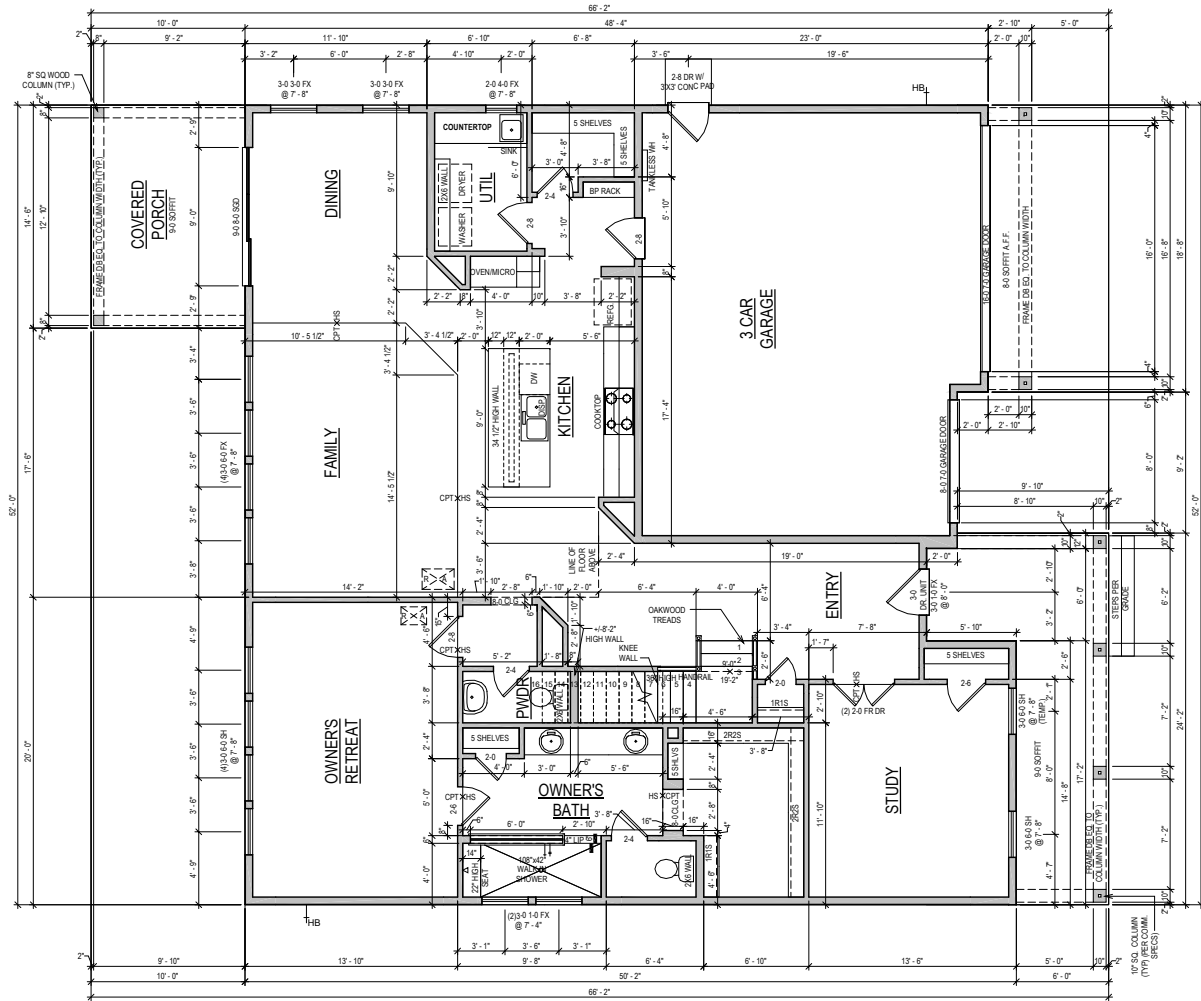
FIRST FLOOR
