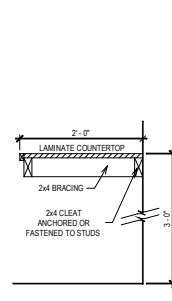
COUNTERTOP DETAIL SCALE: 1/2" = 1'-0"
