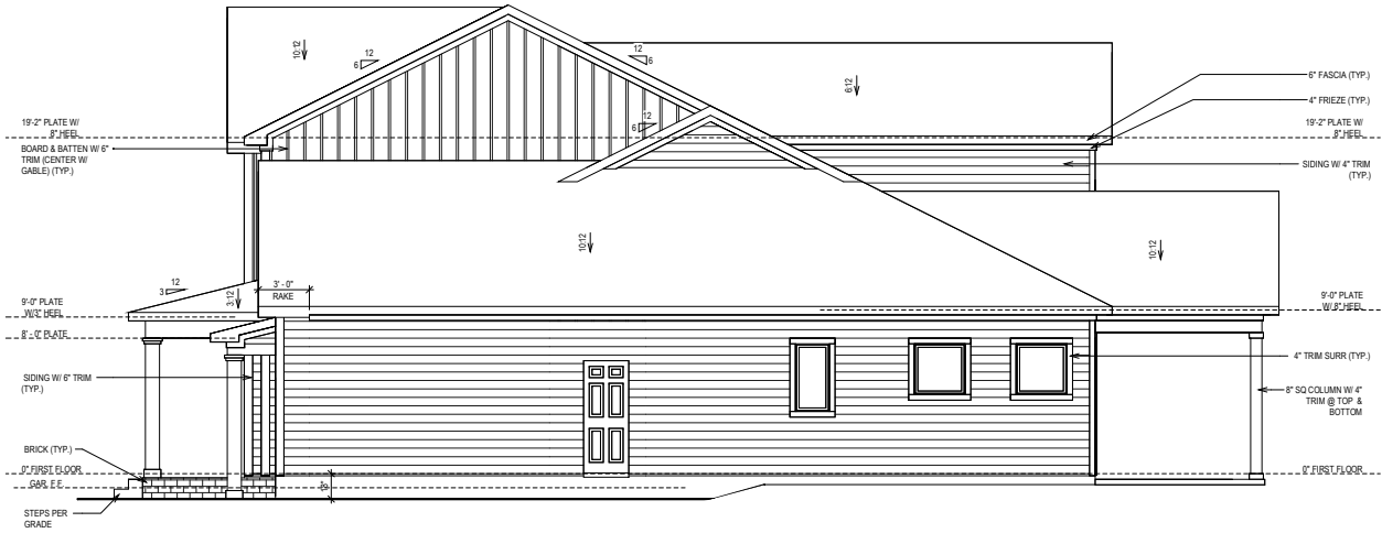
SIDE ELEVATION
