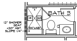
SHOWER W/ SEAT I.L.O. TUB AT BATH 3
