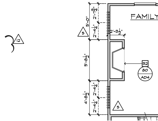
FIREPLACE AT FAMILY
