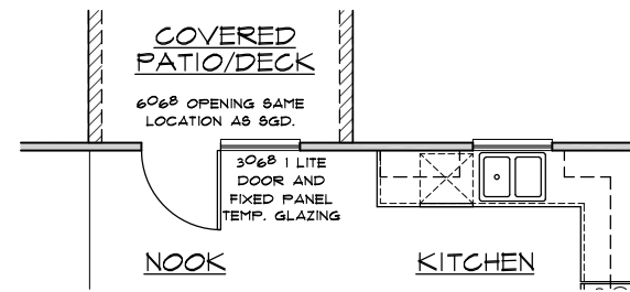
SINGLE LITE DOOR W/ FIXED PANEL AT COVERED/EXTENDED COVERED PATIO/DECK
