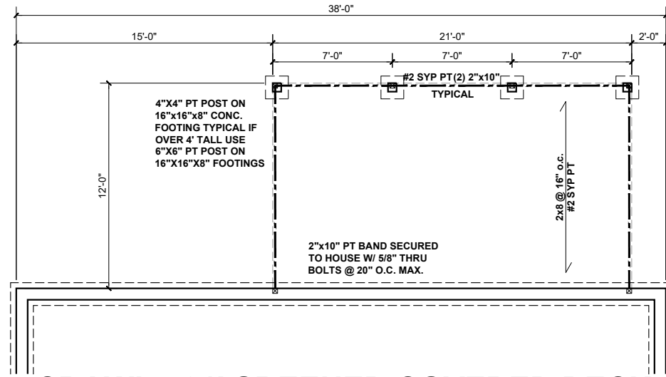
CRAWL - 21' SREENED COVERED DECK SCALE: 1/8" = 1'-0"
