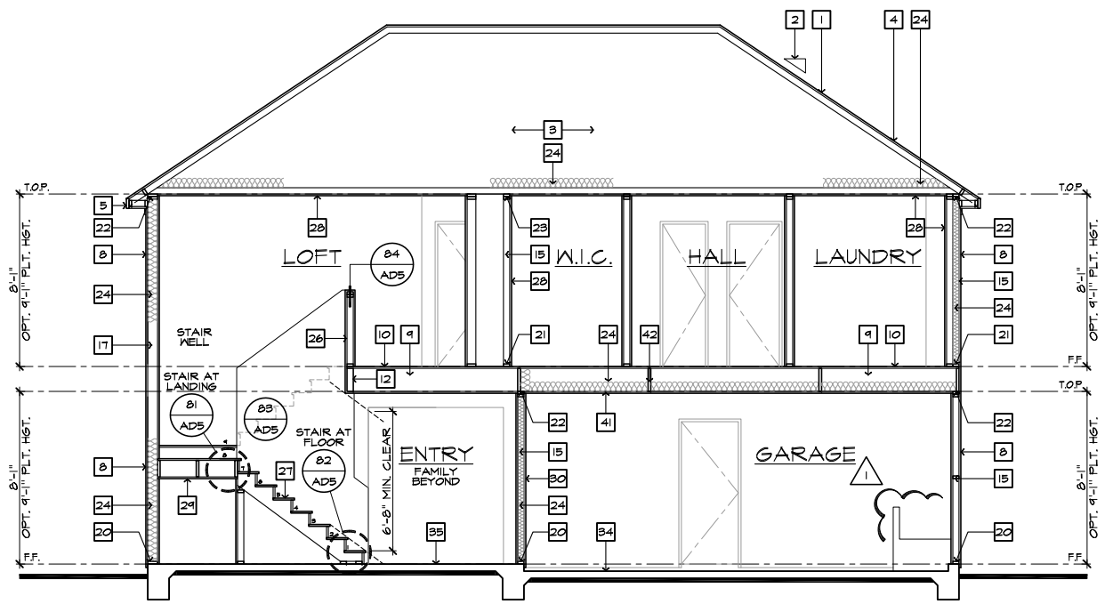
SECTION "A"
