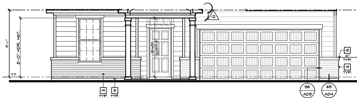
PARTIAL FRONT ELEVATION 'A' AT OPTIONAL 9'-1" PLT. HGT. W/ BRICK OPT. SCALE 1/4"=1'-0" (22"X34") - 1/8"=1'-0" (11"X17")
