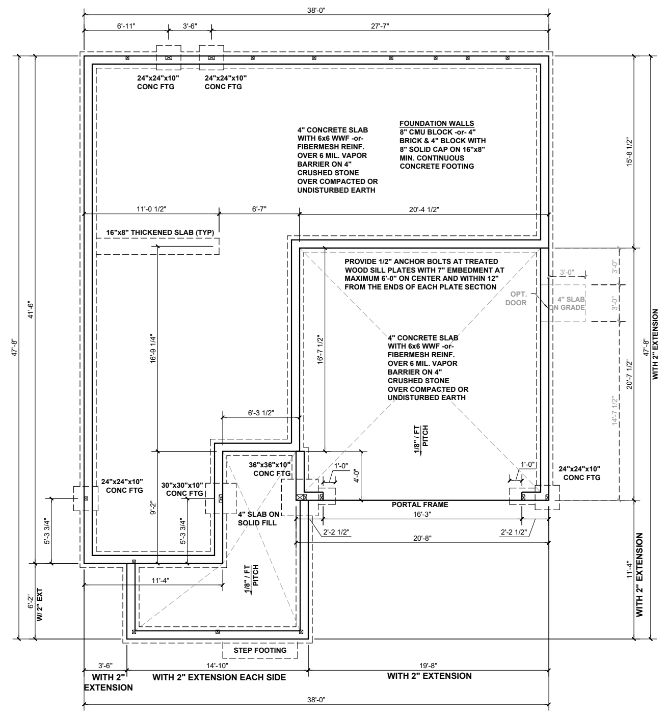
STEM WALL FOUNDATION PLAN - 'C' SCALE: 1/8"=1'-0"
