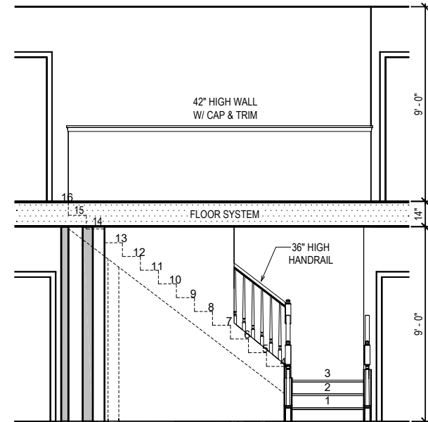
STAIR SECTION
