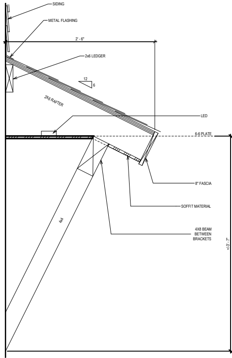
AWNING DETAIL W/ BEAM SCALE: 1" = 1'-0"
