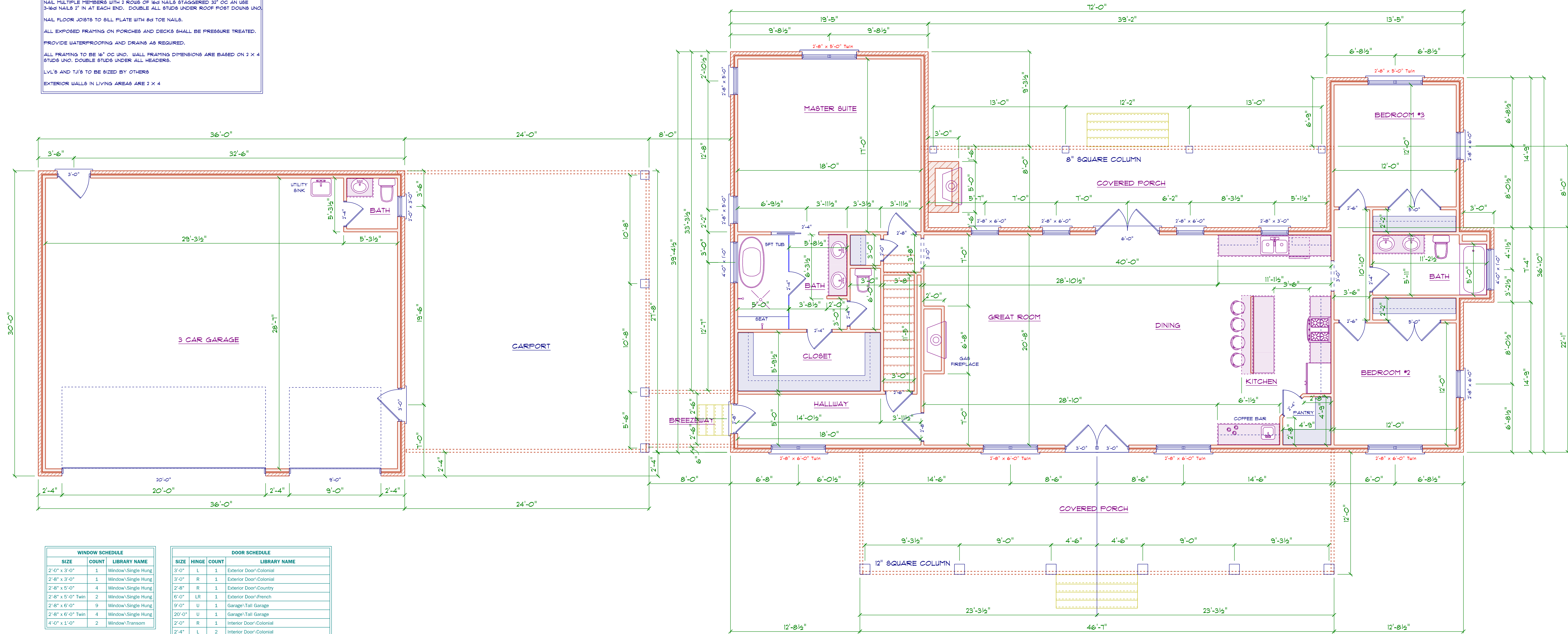
1ST FLOOR PLAN SCALE: 1" = 3/16"
