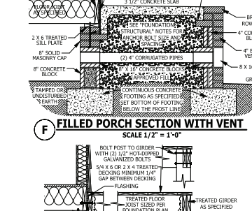
F FILLED PORCH SECTION WITH VENT SCALE 1/2" = 1'-0"
