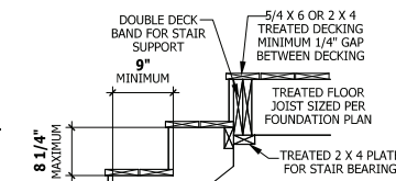
FIGURE AM110 TYPICAL DECK STAIR DETAIL SCALE 3/4" = 1'-0"
