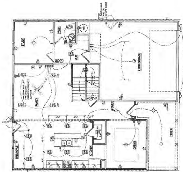
ELEVATION - B FIRST FLOOR ELECTRICAL PLAN SCALE 1/8" = 1'-0" (NOT TO SCALE)
