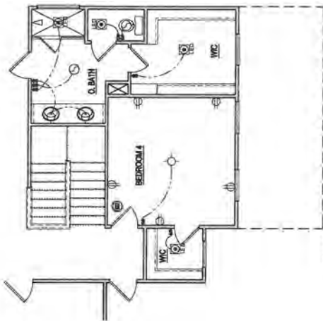
ELEVATION 'B' OPT. BEDROOM 4 LAYOUT SCALE: 1/8" = 1'-0" (SHEET SIZE)
