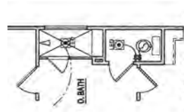
OPT. SPA SHOWER SCALE: 1/8" = 1'-0" (SHEET SIZE)
