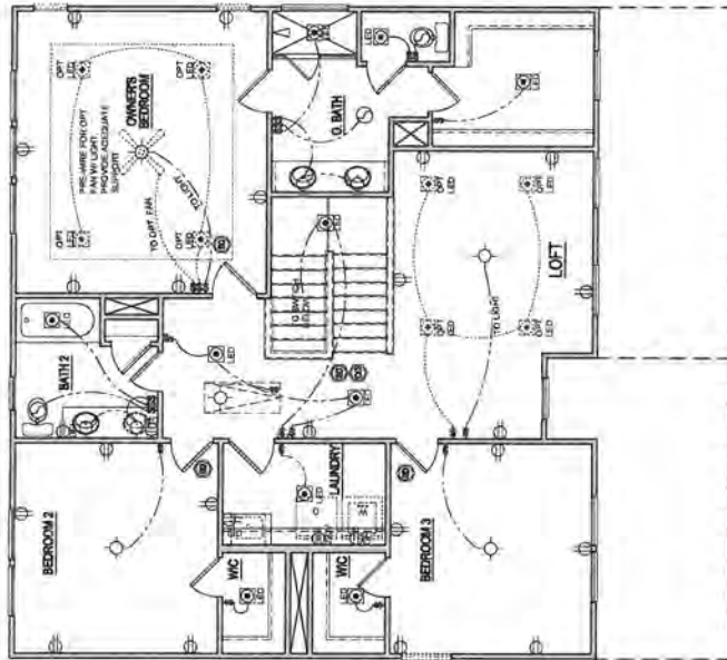
ELEVATION - B SECOND FLOOR ELECTRICAL PLAN SCALE: 1/8" = 1'-0" (SHEET SIZE)
