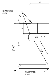
TRELLIS DETAIL
