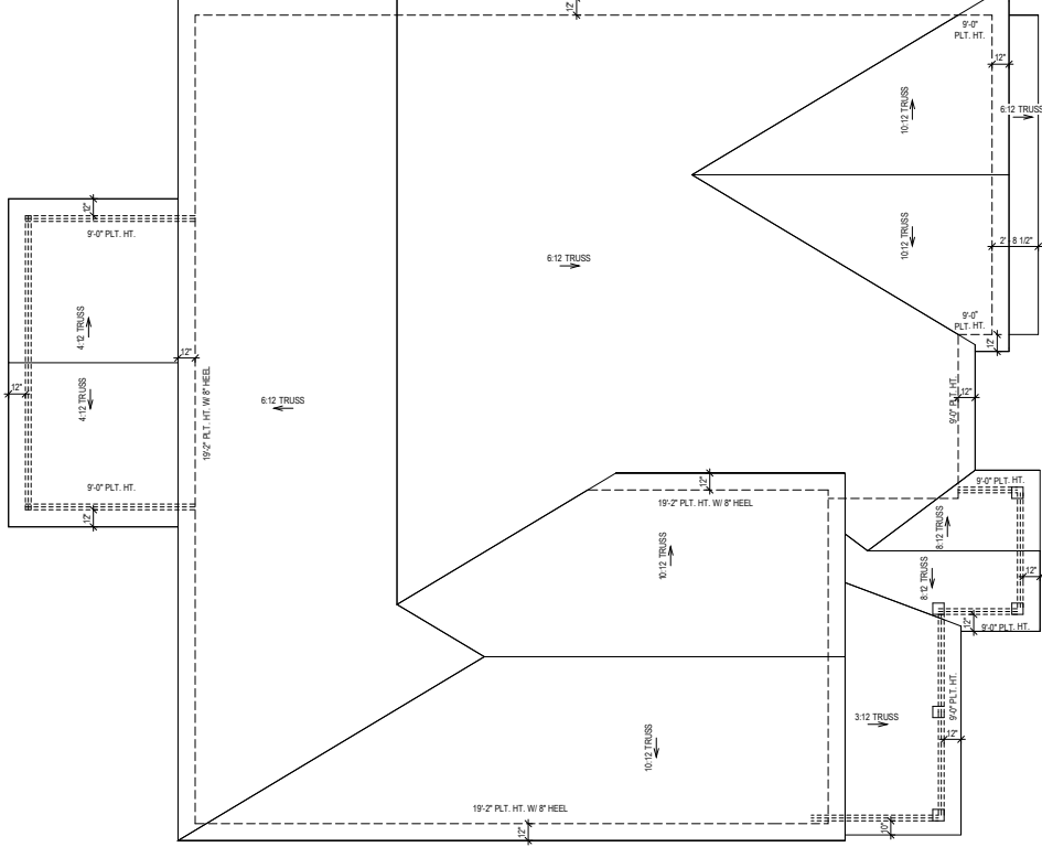
ROOF PLAN
