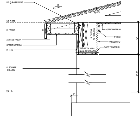
CORNICE DETAIL "A"
