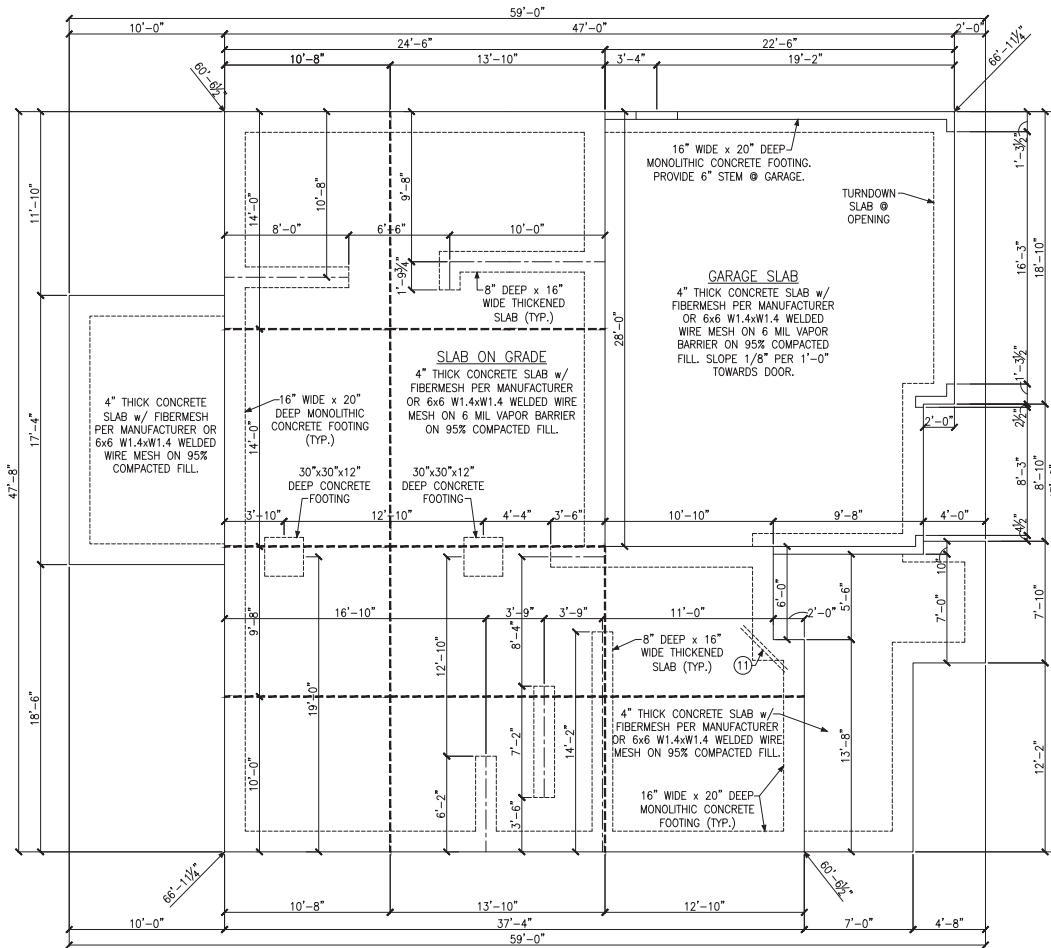
MONOLITHIC SLAB FOUNDATION PLAN
