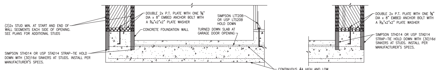
(C) METHOD CS-PF: ENGINEERED PORTAL FRAME WITH HOLD-DOWNS
