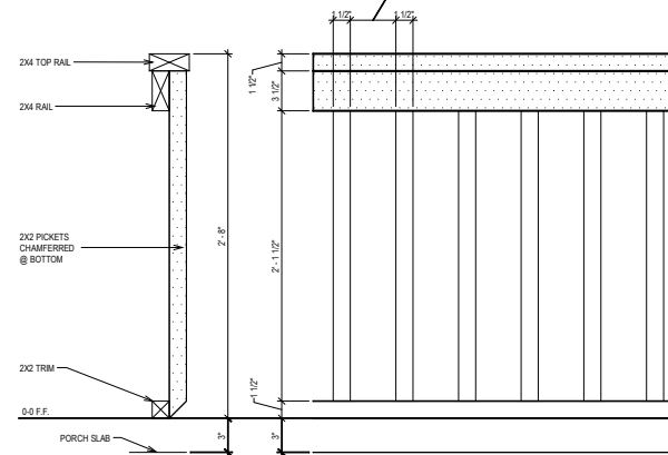
RAILING DETAIL
