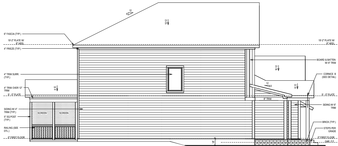
SIDE ELEVATION
