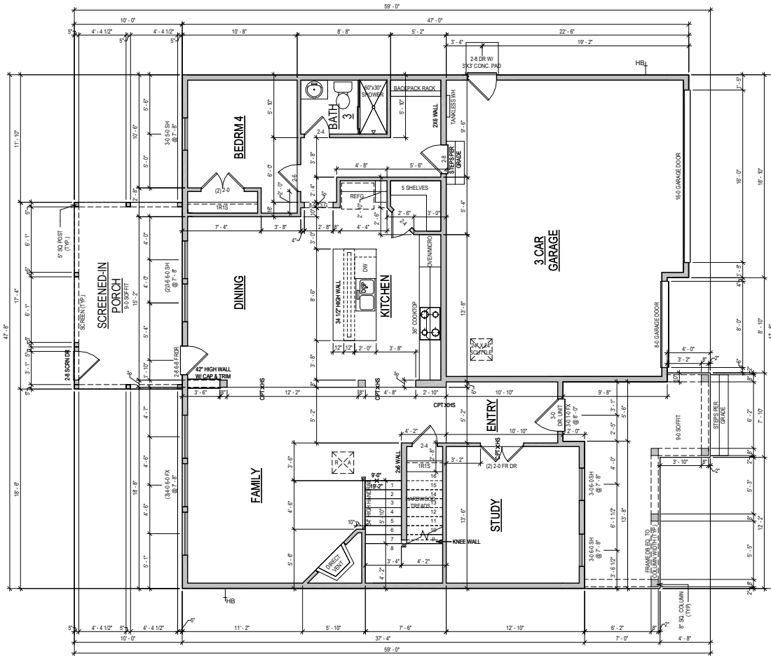
FIRST FLOOR
