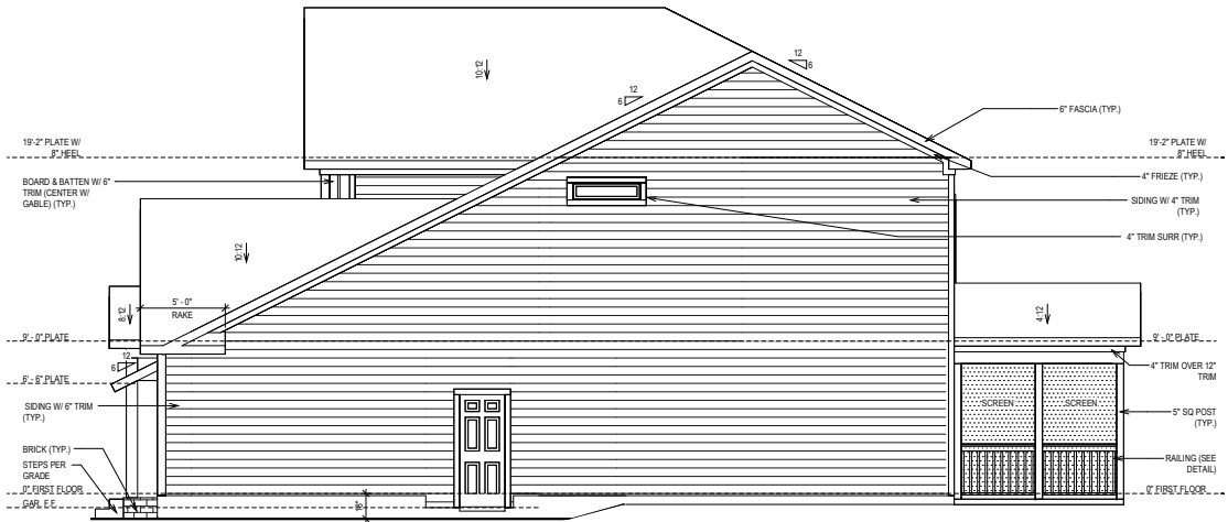
SIDE ELEVATION
