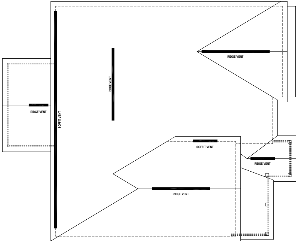
ROOF PLAN W/ SCREENED-IN PORCH CALCS
