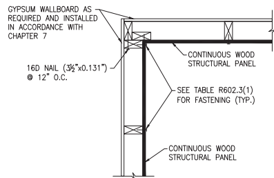
J TYPICAL EXTERIOR CORNER FRAMING INSIDE CORNER DETAIL
