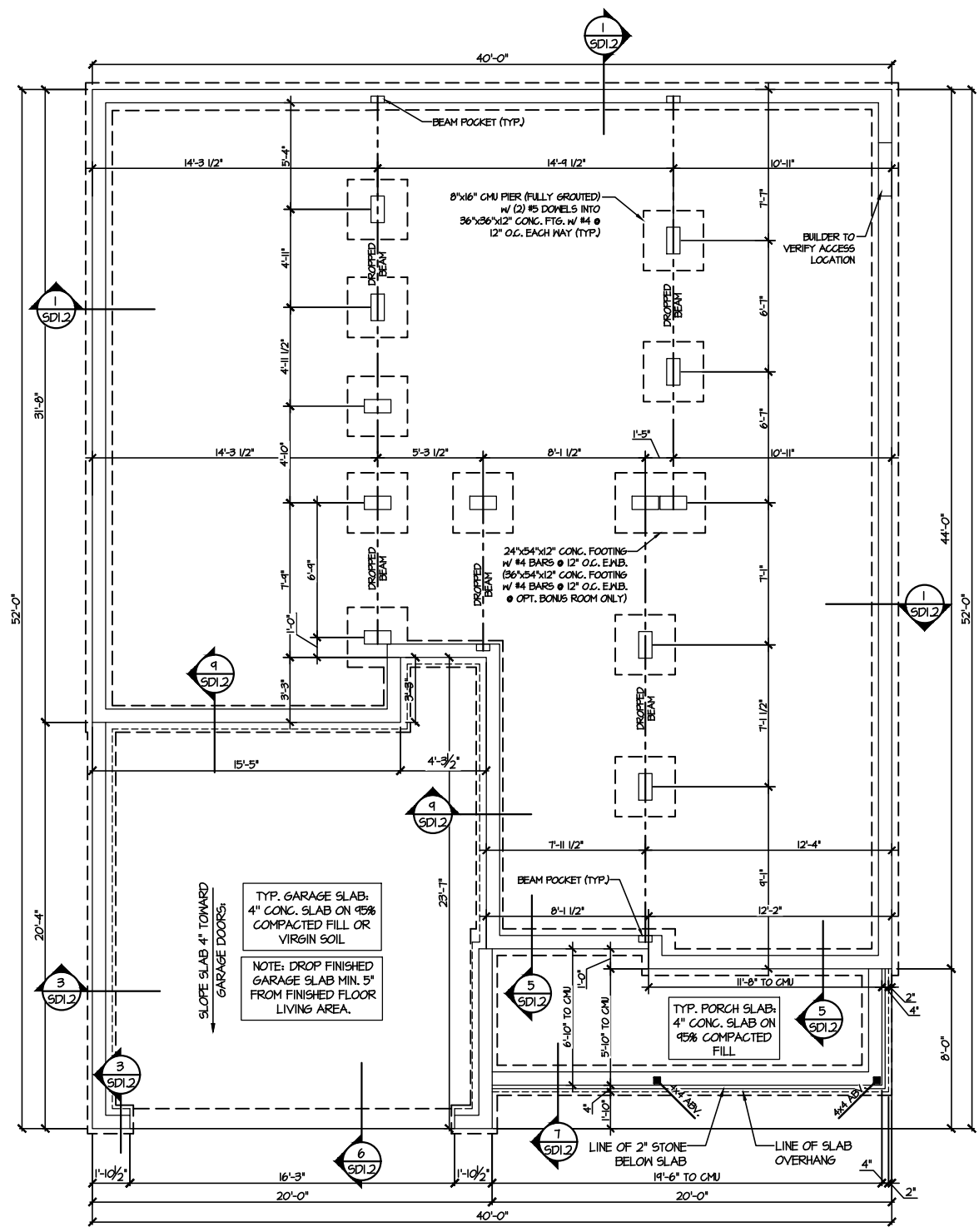
CRAWL SPACE FOUNDATION PLAN SCALE: 1/8"=1'-0"
