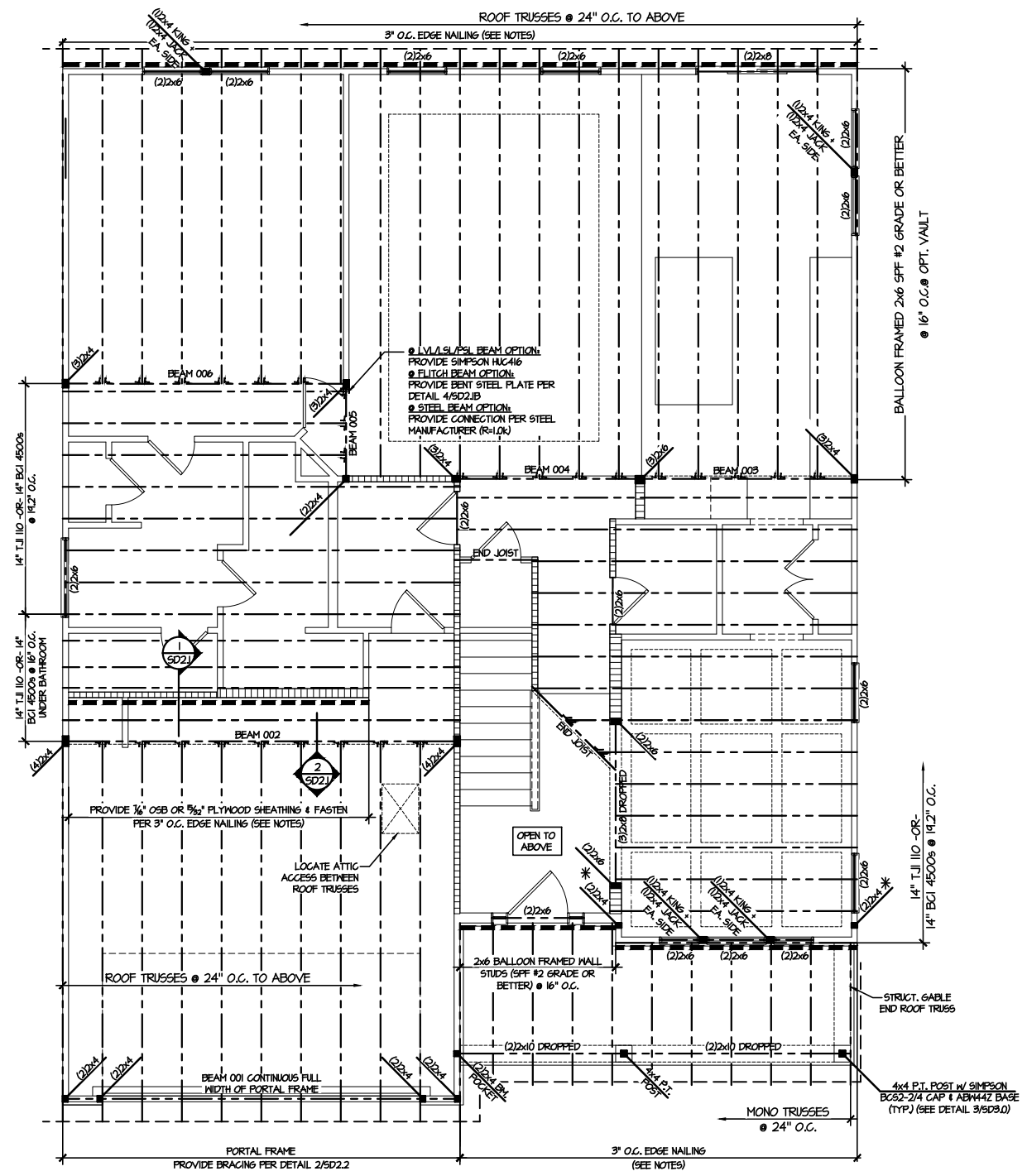
2ND FLOOR FRAMING PLAN SCALE: 1/8"=1'-0"
