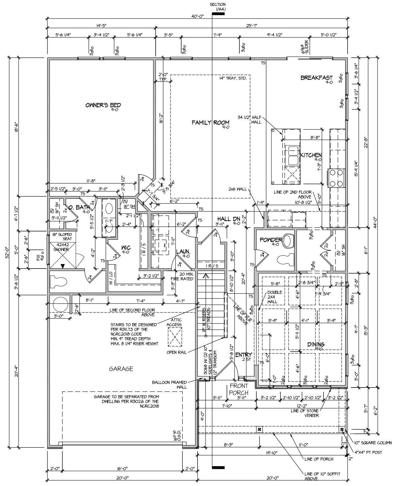
ELEVATION 4 FIRST FLOOR PLAN SCALE: 1/8" = 1'-0"
