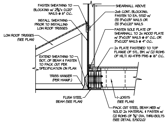
2 SHEAR TRANSFER DETAIL @ EXTERIOR SHEARWALL ABOVE
