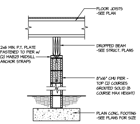
8 TYPICAL CRAWLSPACE FOUNDATION @ INTERIOR PIER SCALE: 3/8"=1'-0"
