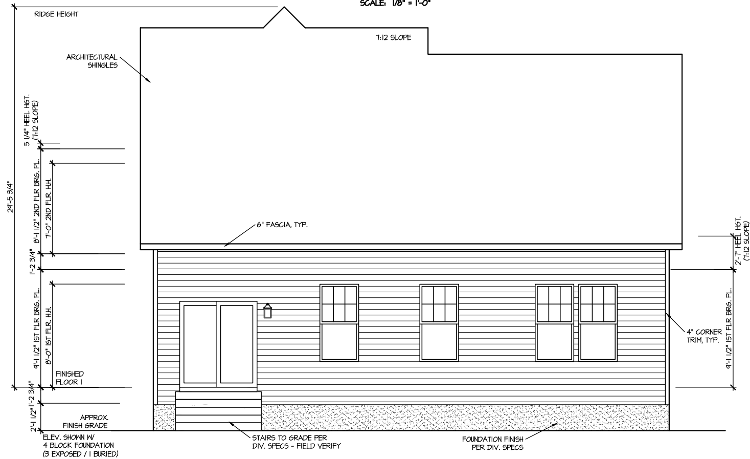
REAR ELEVATION 4
