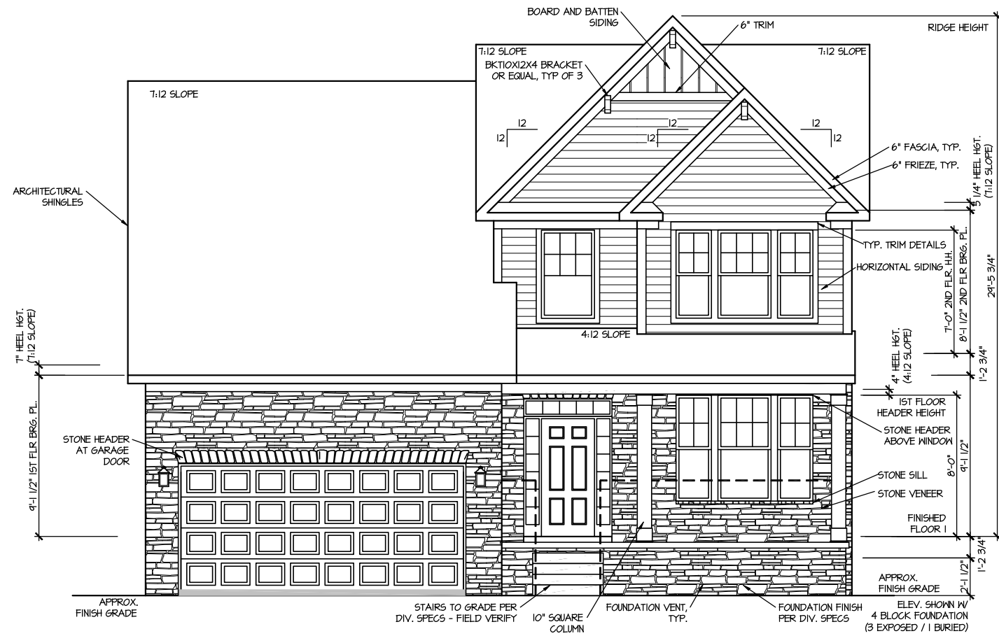
FRONT ELEVATION 4
