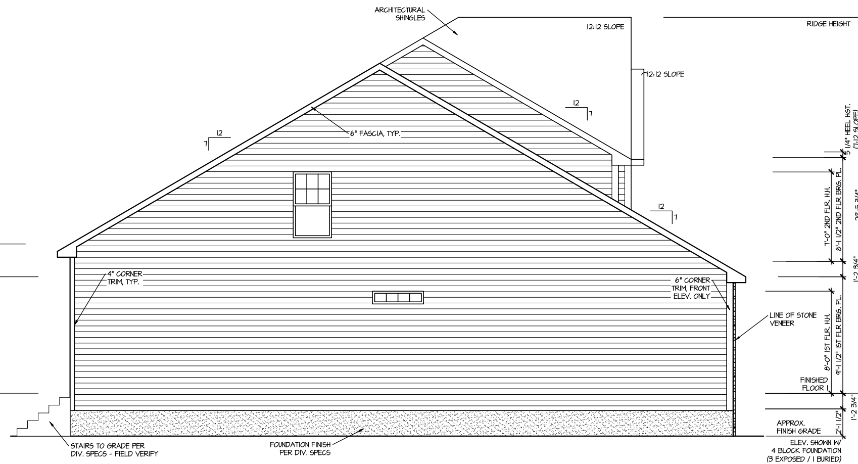
LEFT ELEVATION 4
