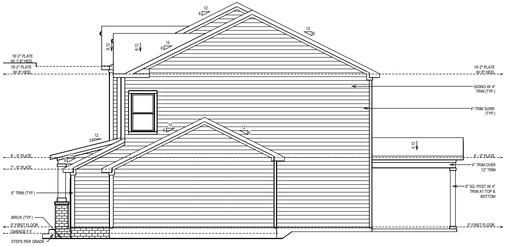
SIDE ELEVATION
