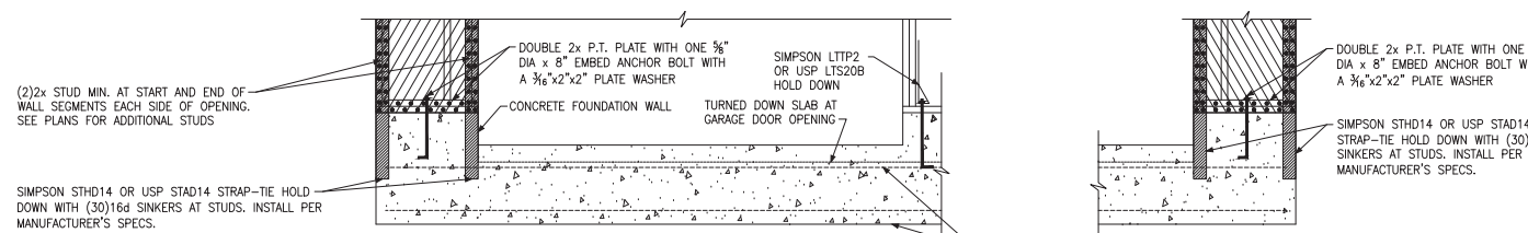
(C) METHOD CS-EPF: ENGINEERED PORTAL FRAME WITH HOLD-DOWNS CONTINUOUS #4 HIGH AND LOW. PROVIDE MIN 24\"/>
