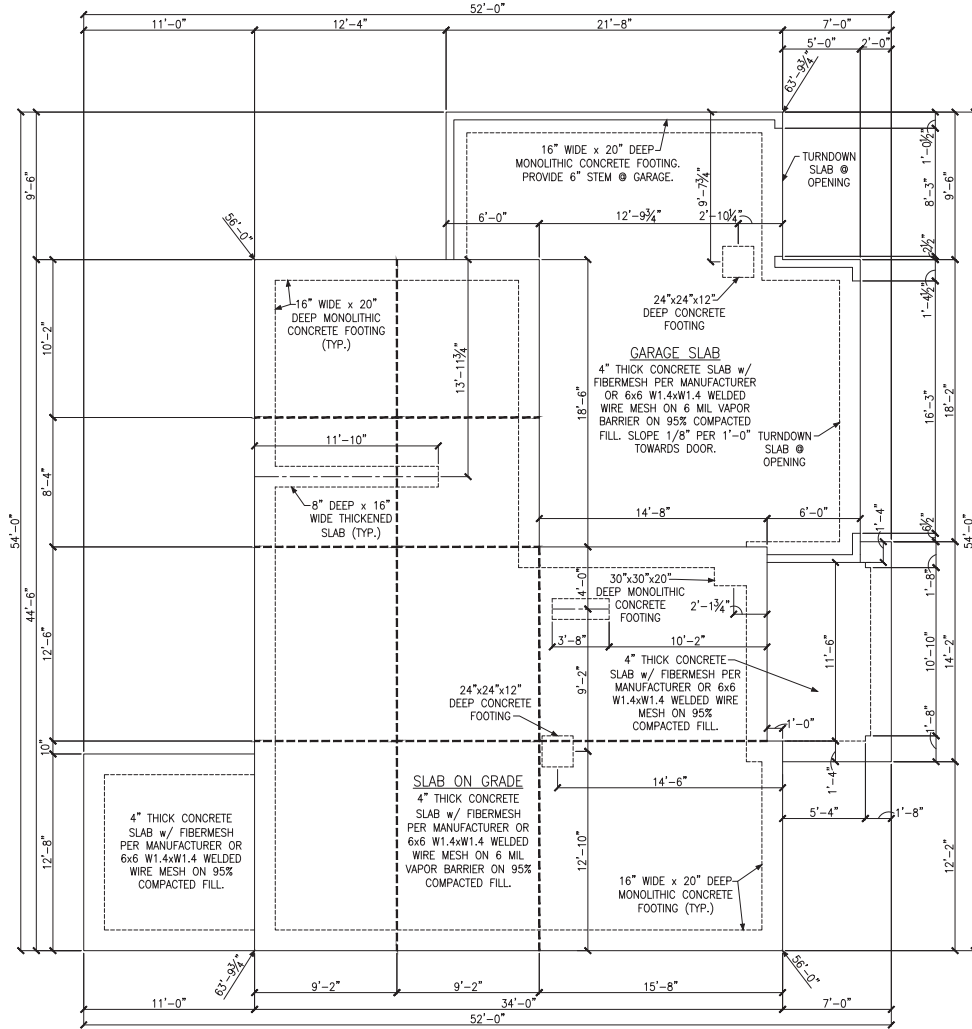
MONOLITHIC SLAB FOUNDATION PLAN
