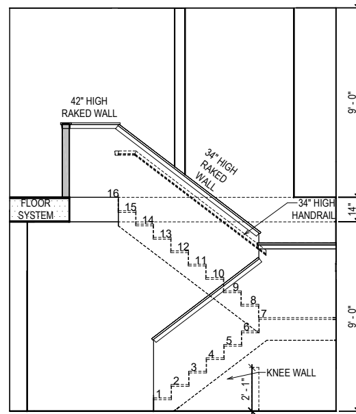
STAIR SECTION
