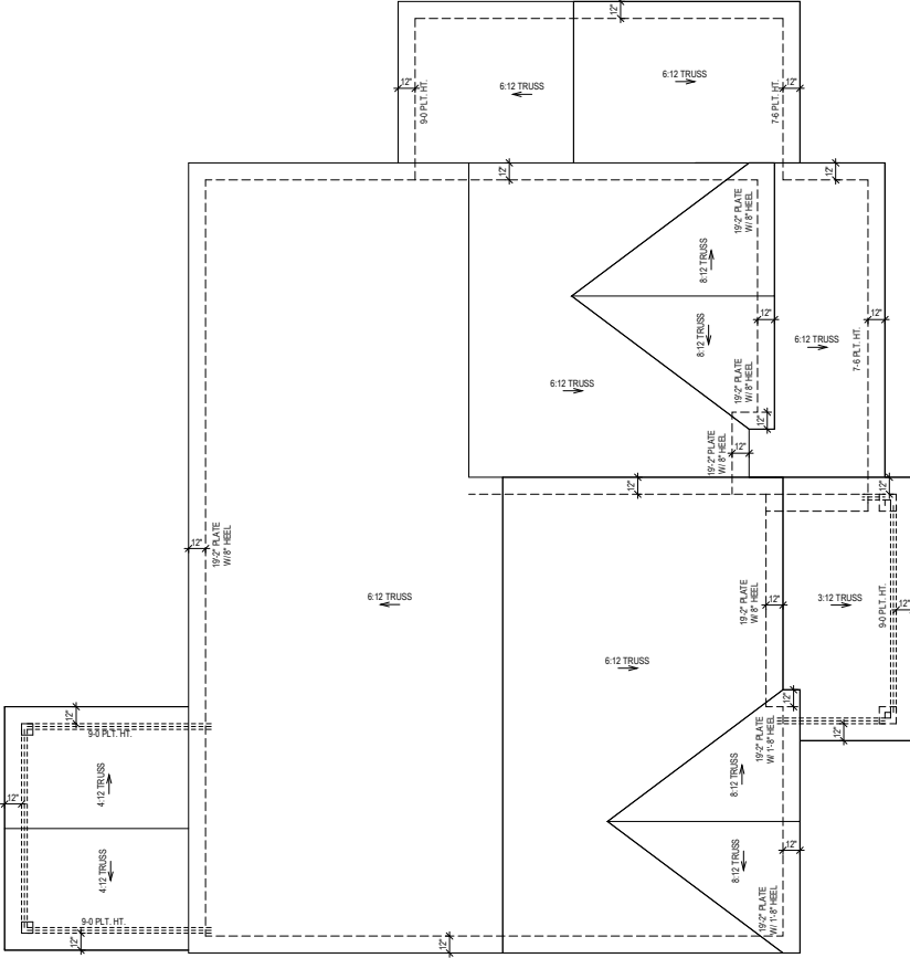
ROOF PLAN
