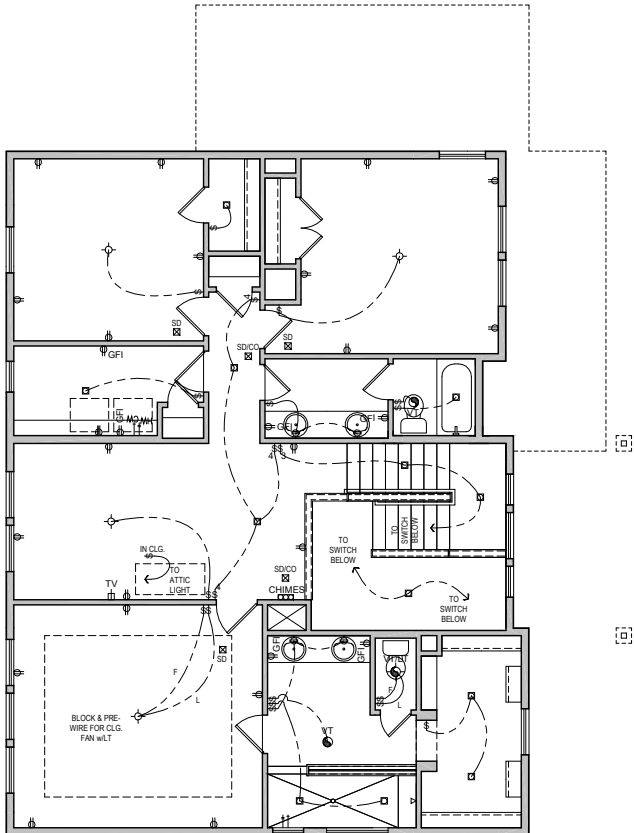
SECOND FLOOR
