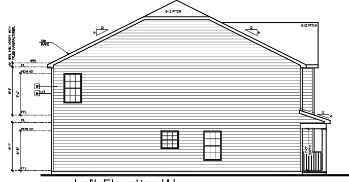
Left Elevation 'A' SCALE: 1/4"=1'-0" AT 22'X34' LAYOUT 1/8"=1'-0" AT 11'X11' LAYOUT
