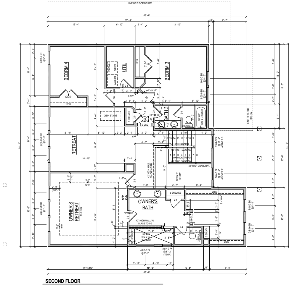
SECOND FLOOR
