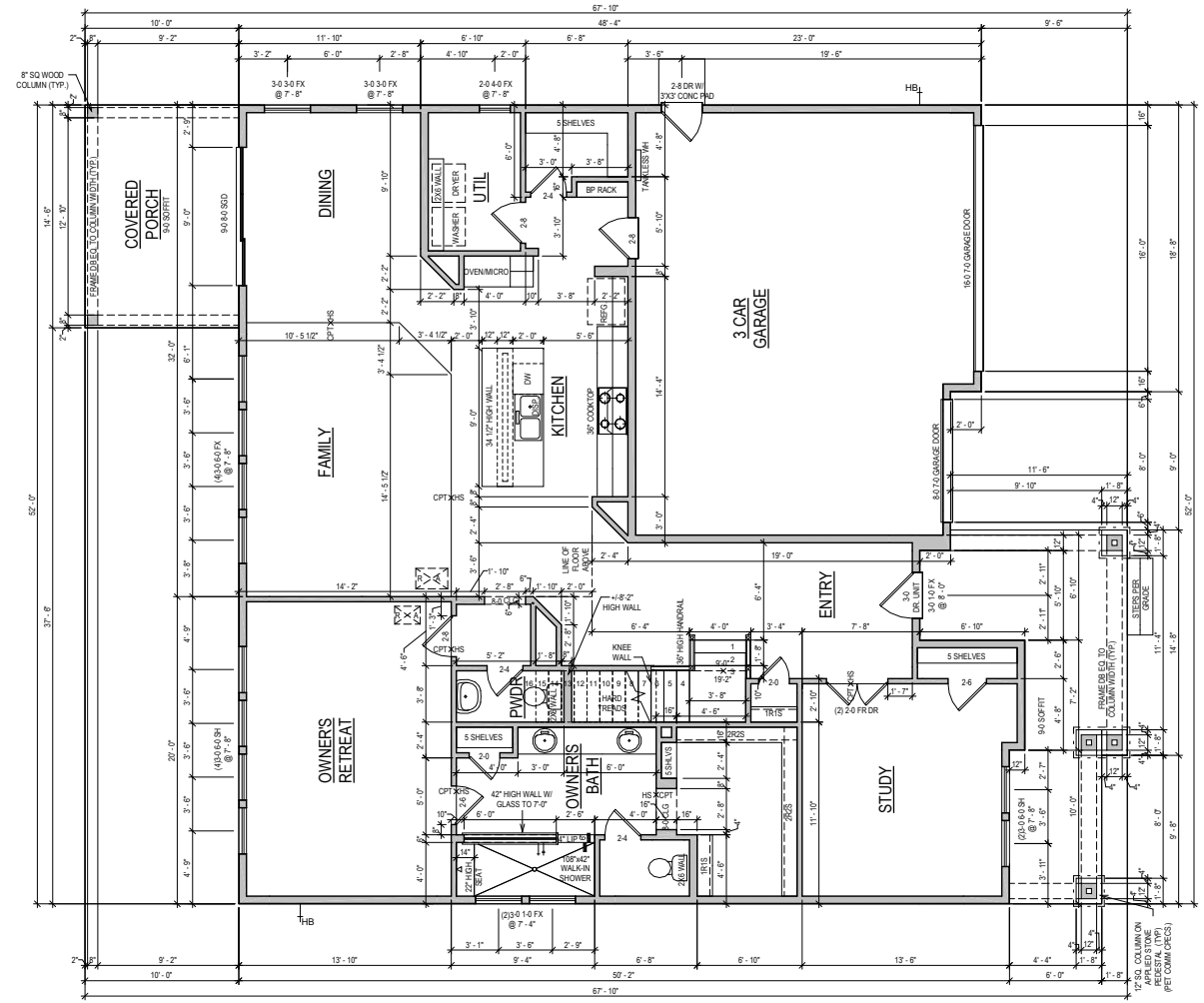
FIRST FLOOR
