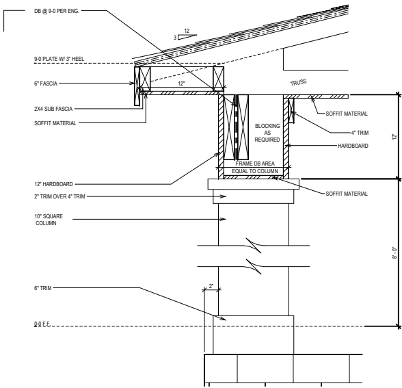
CORNICE DETAIL "A"
