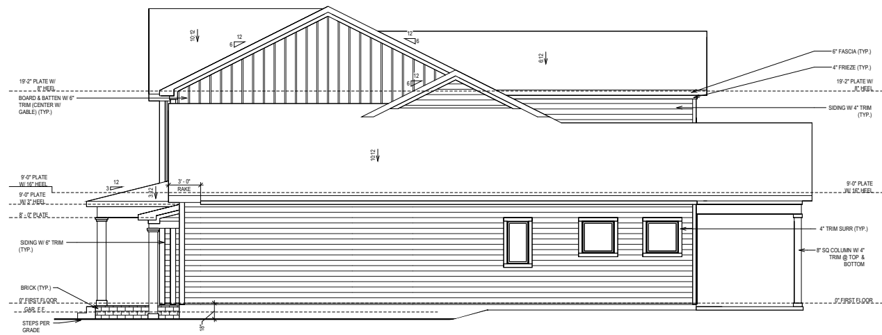
SIDE ELEVATION
