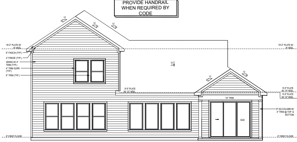
REAR ELEVATION
