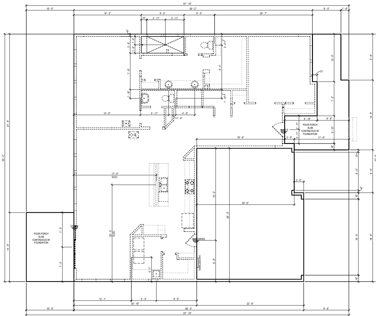
FIRST FLOOR
