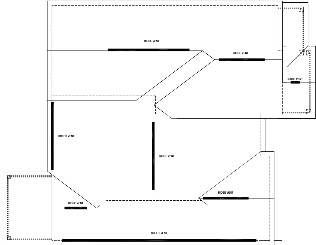
ROOF PLAN
