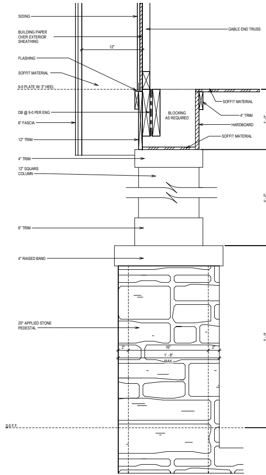
CORNICE B DETAIL
