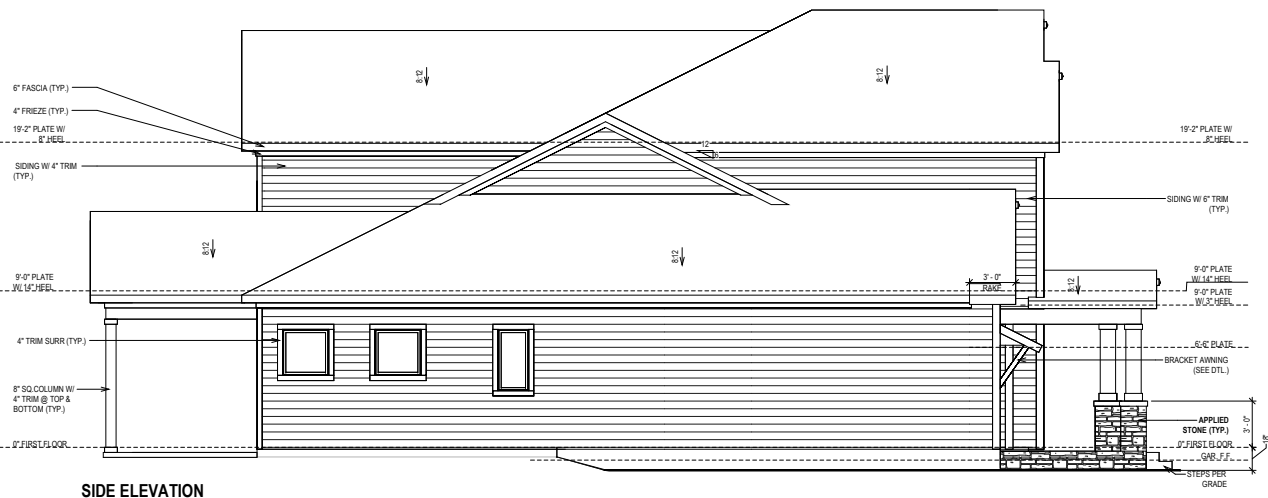
SIDE ELEVATION
