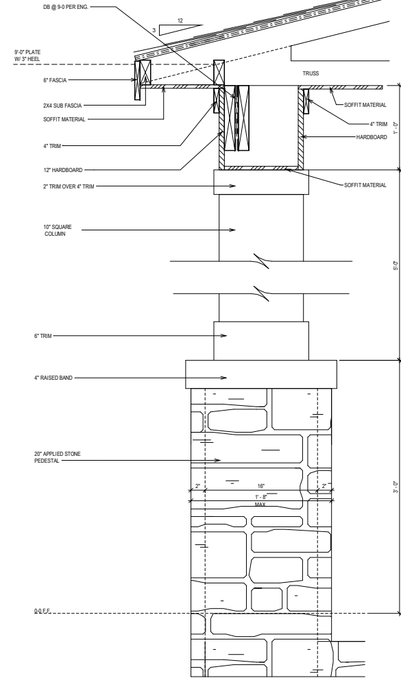
CORNICE A DETAIL
