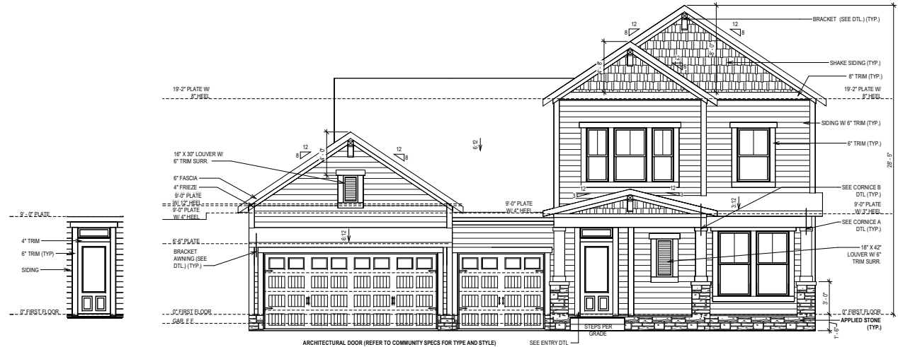
FRONT ELEVATION "B"
