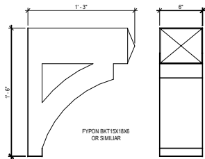
BRACKET DETAIL
