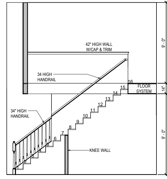
STAIR SECTION
