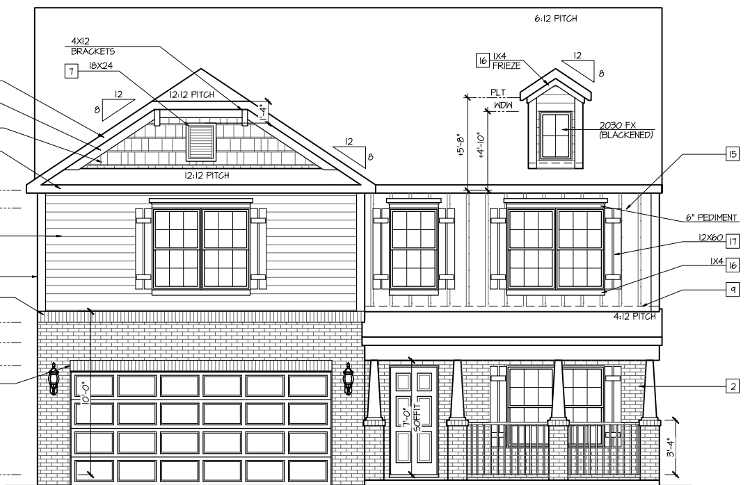
Front Elevation 'B' SCALE: 1/4"=1'-0" AT 22'X34" LAYOUT 1/8"=1'-0" AT 11'X11" LAYOUT
