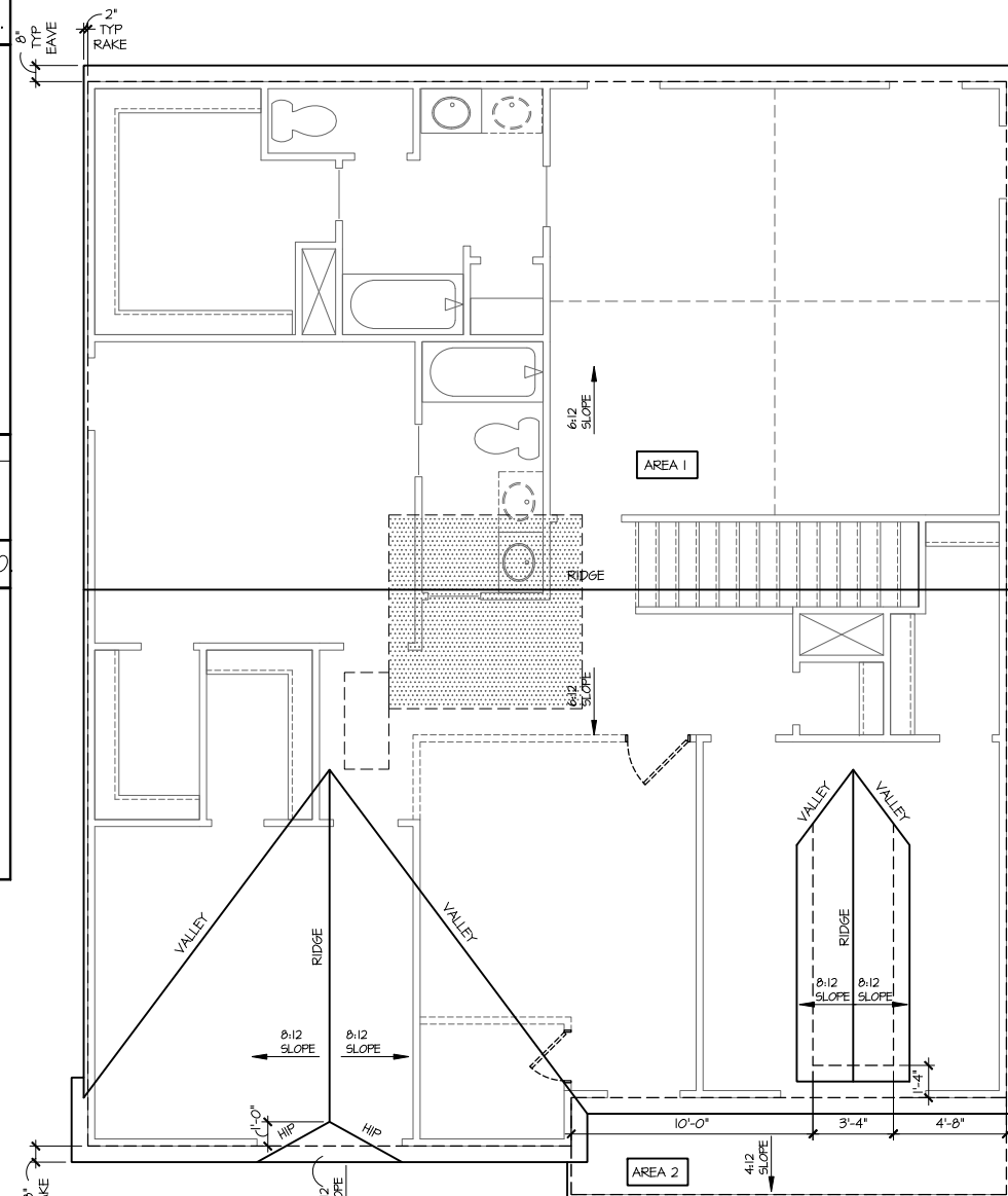
Roof Plan 'B' SCALE: 1/4"=1'-0" AT 22'X34" LAYOUT 1/8"=1'-0" AT 11'X11" LAYOUT
