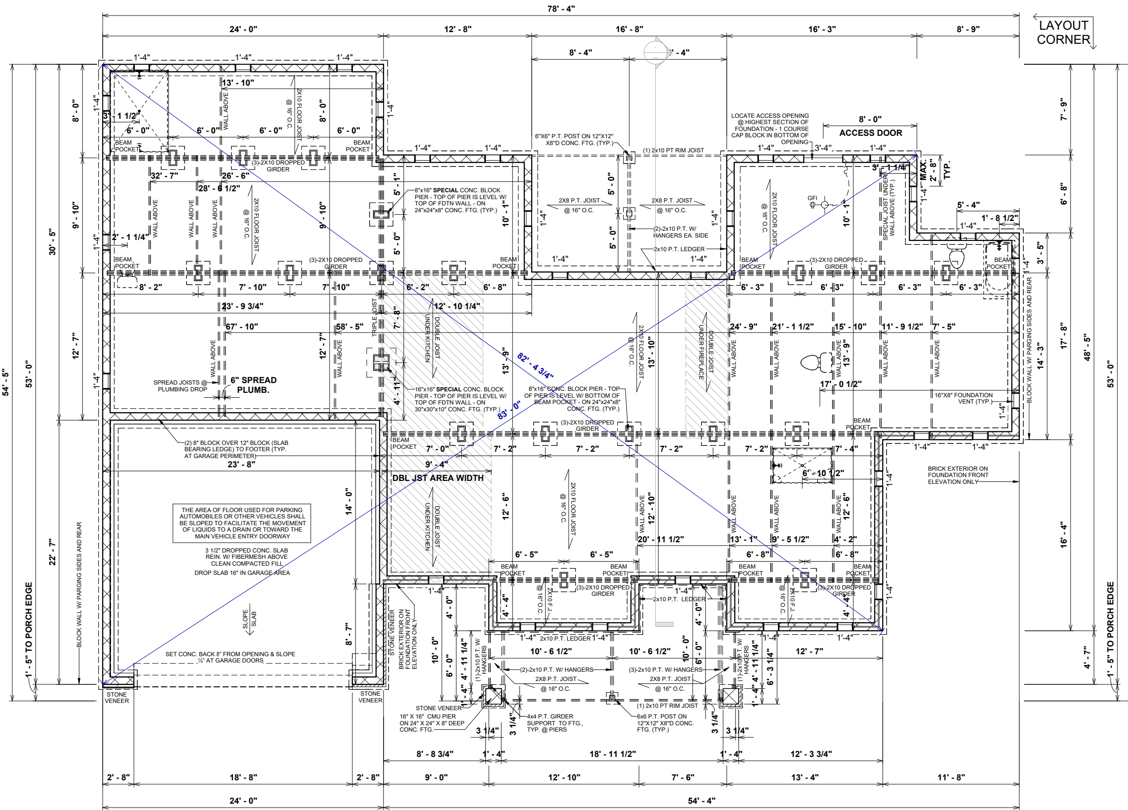
1 FOUNDATION PLAN 1/8" = 1'-0"
