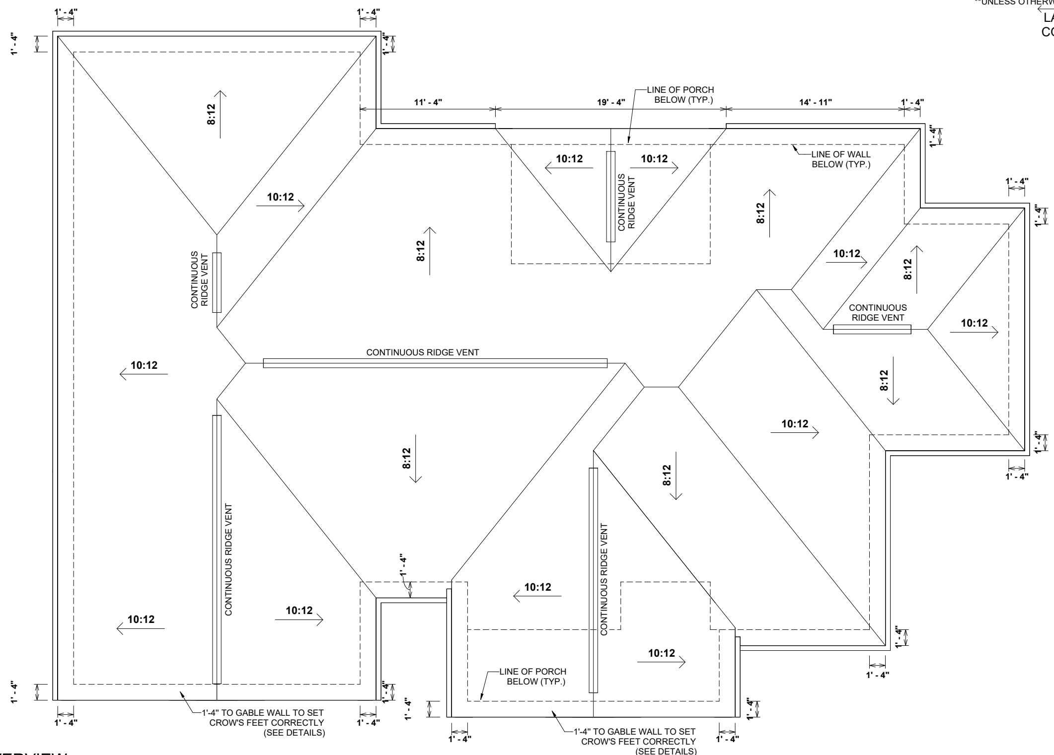
1 ROOF OVERVIEW 1/8" = 1'-0"
