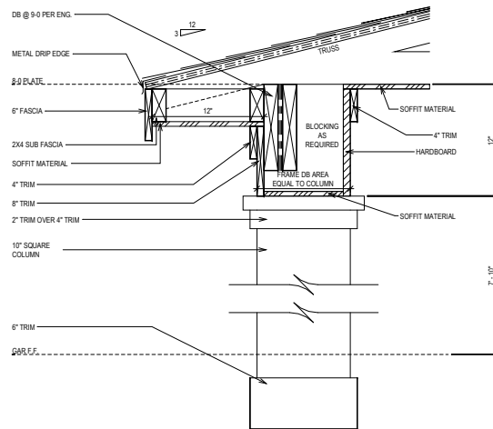
CORNICE DETAIL "B"
