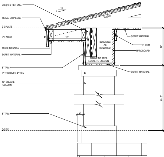
CORNICE DETAIL "A"
