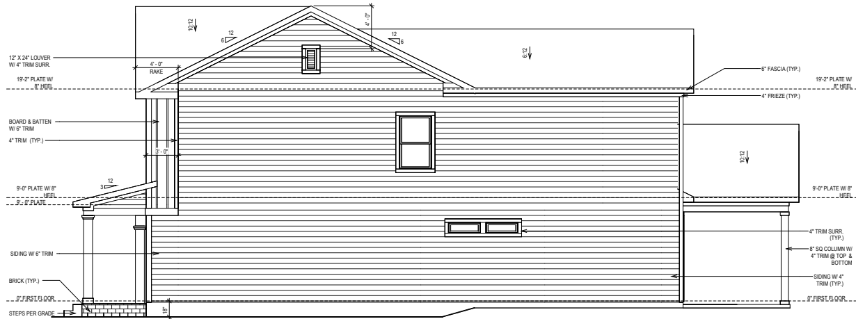
SIDE ELEVATION
