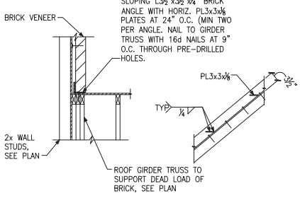
D TRUSS DETAIL
