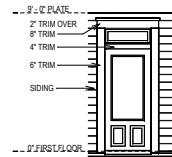
ENTRY DETAIL
