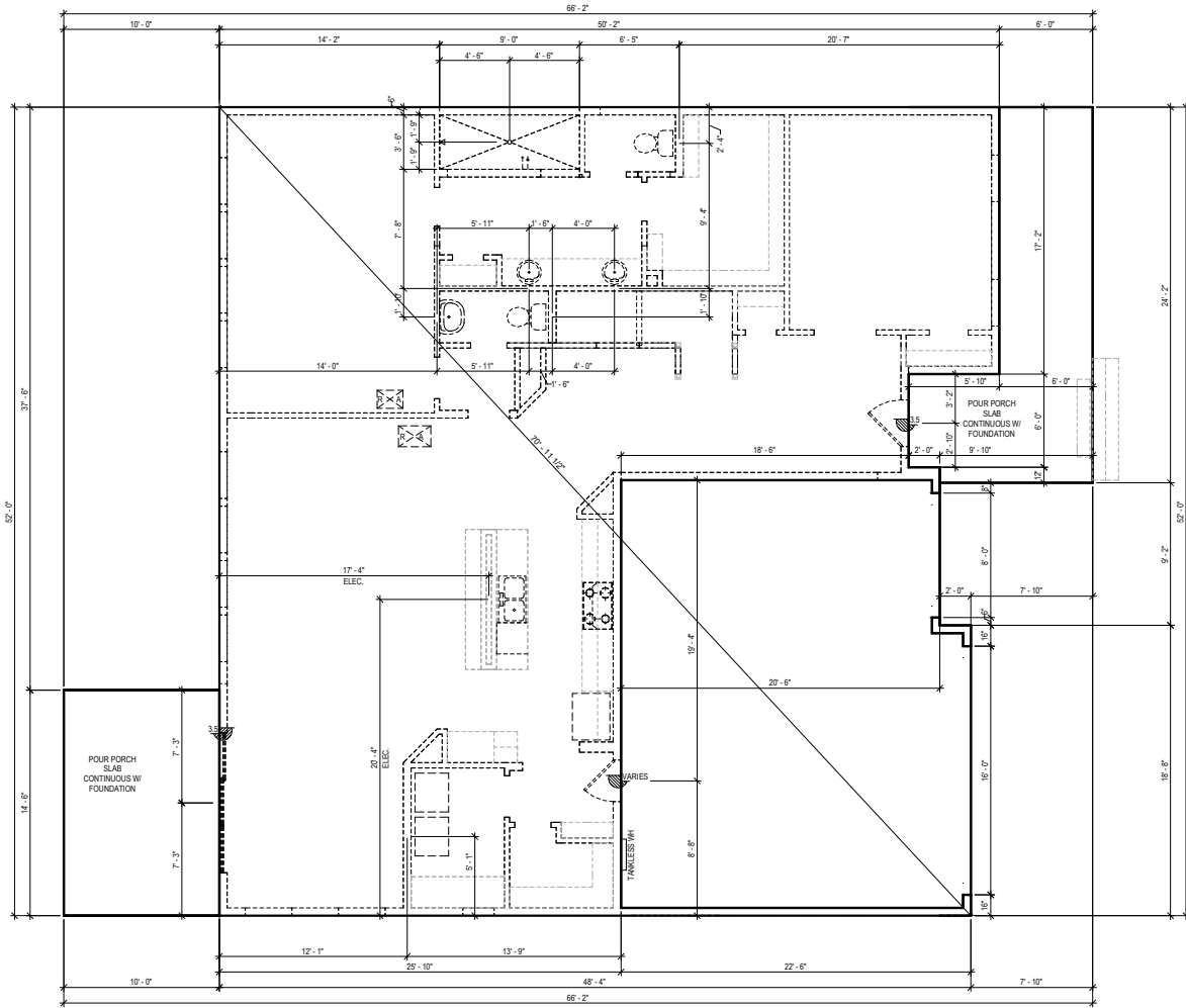
FIRST FLOOR
