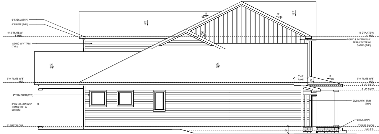
SIDE ELEVATION
