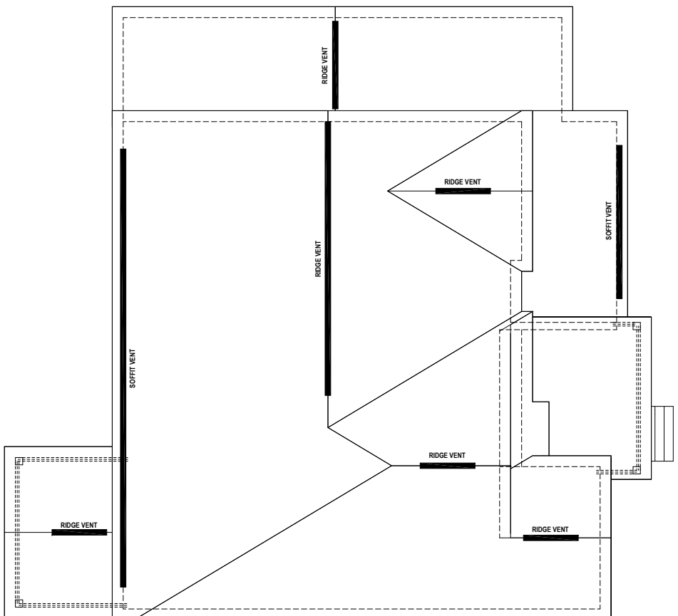
ROOF PLAN W/ COVERED PORCH CALCS
