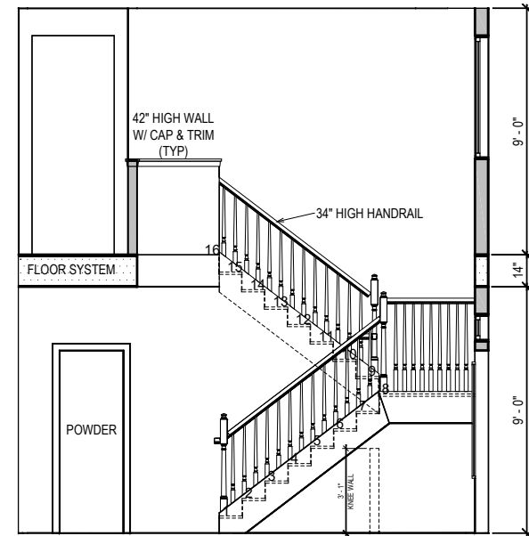
STAIR SECTION W/ RAIL
