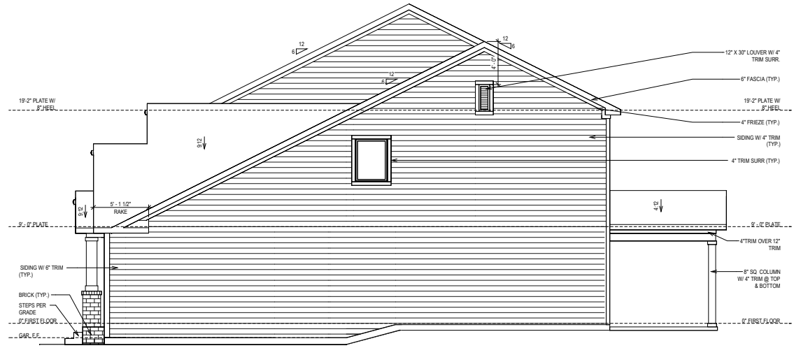
SIDE ELEVATION
