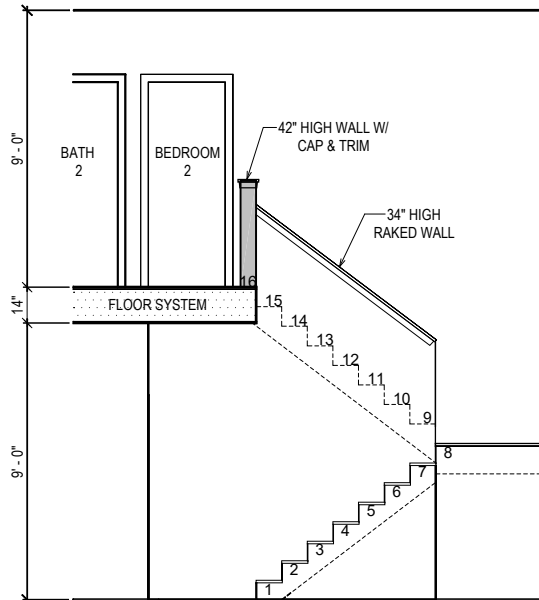
STAIR SECTION
