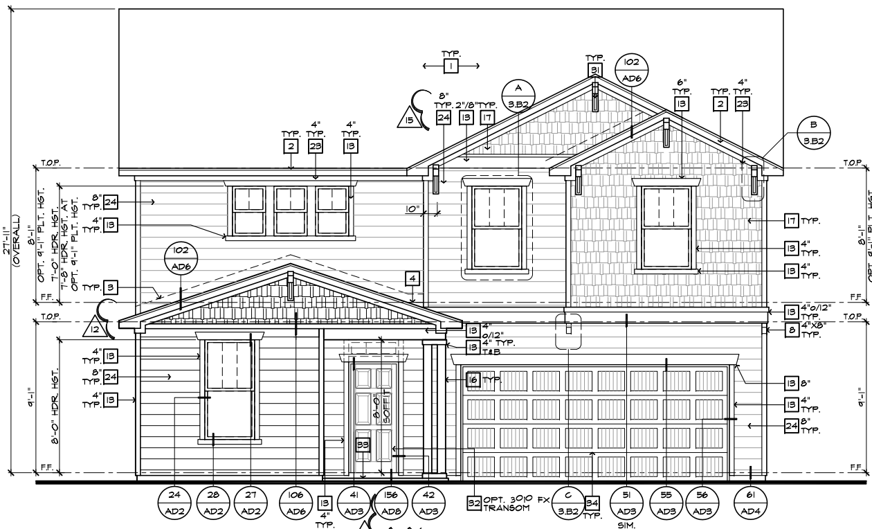
FRONT ELEVATION 'B' AT OPTIONAL 9'-1" PLT. HGT.
