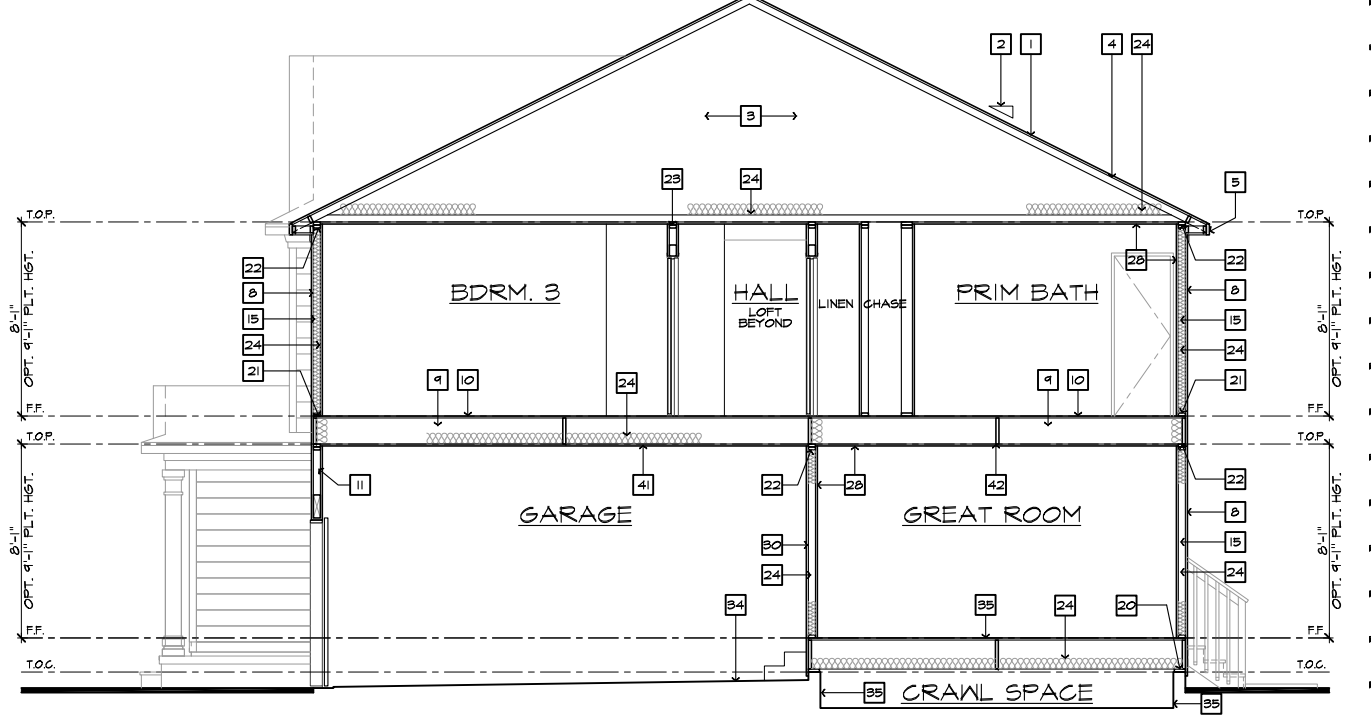
SECTION "B"
