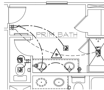
DELUXE PRIM BATH AT PRIM BATH
