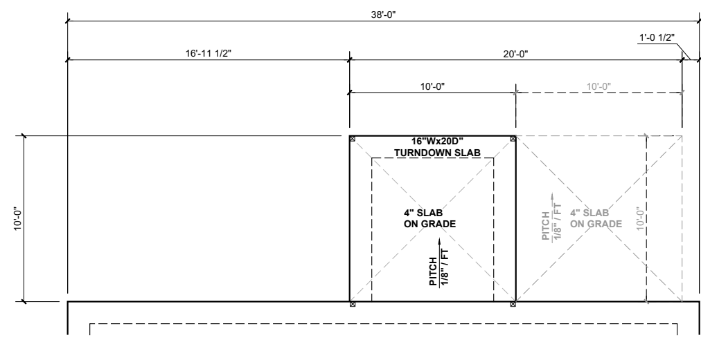
SLAB FDN - 10' COVERED SCREENED PATIO SCALE: 1/8" = 1'-0"
