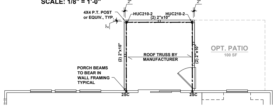
10' COVERED SCREENED PATIO SCALE: 1/8" = 1'-0"
