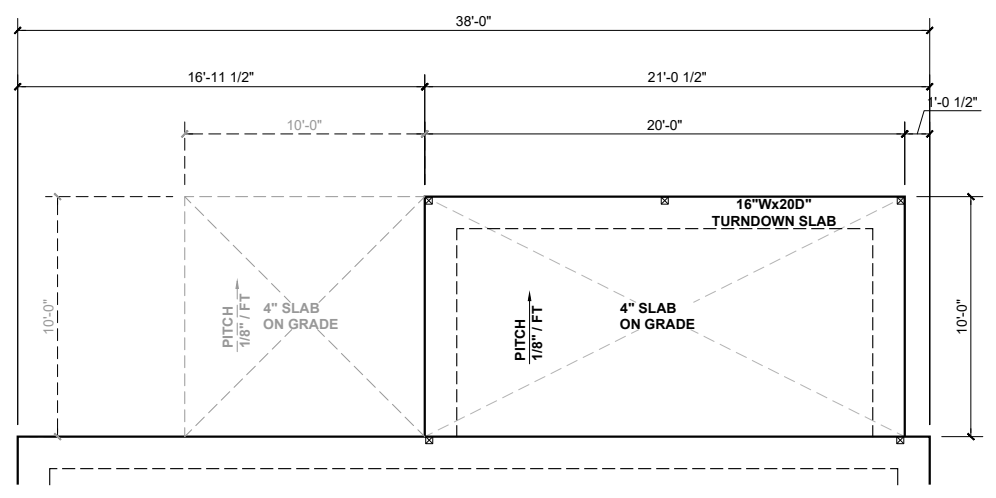
SLAB FDN - EXT. COVERED SCREENED PATIO SCALE: 1/8" = 1'-0"
