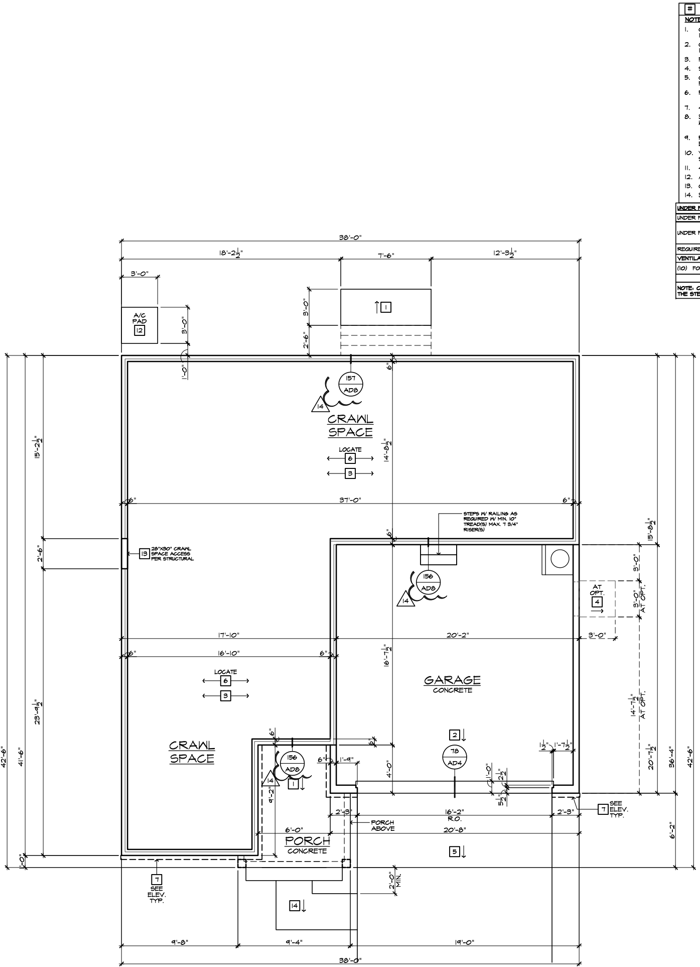
CRAWL SPACE PLAN 'A' SCALE 1/4"=1'-0" (22"X34") - 1/8"=1'-0" (11"X17")
