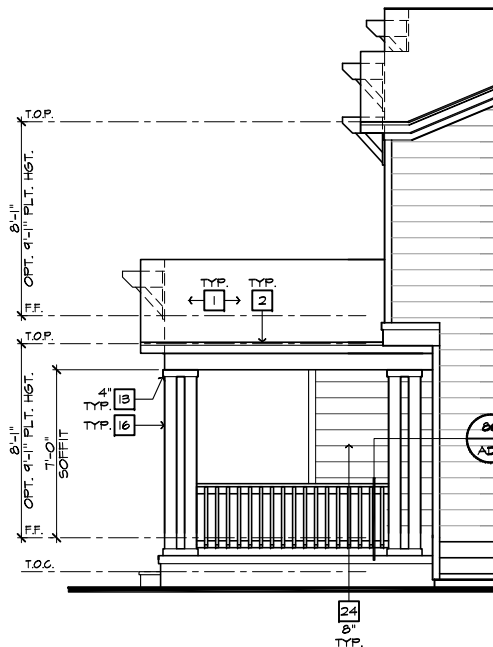
PARTIAL RIGHT ELEVATION 'B' AT OPTIONAL PORCH W/ CRAWL SPACE
