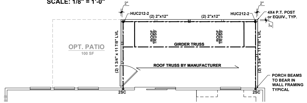
EXT. COVERED SCREENED PATIO SCALE: 1/8" = 1'-0"
