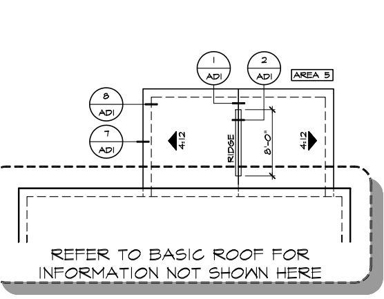
PARTIAL CRAWL SPACE PLAN
