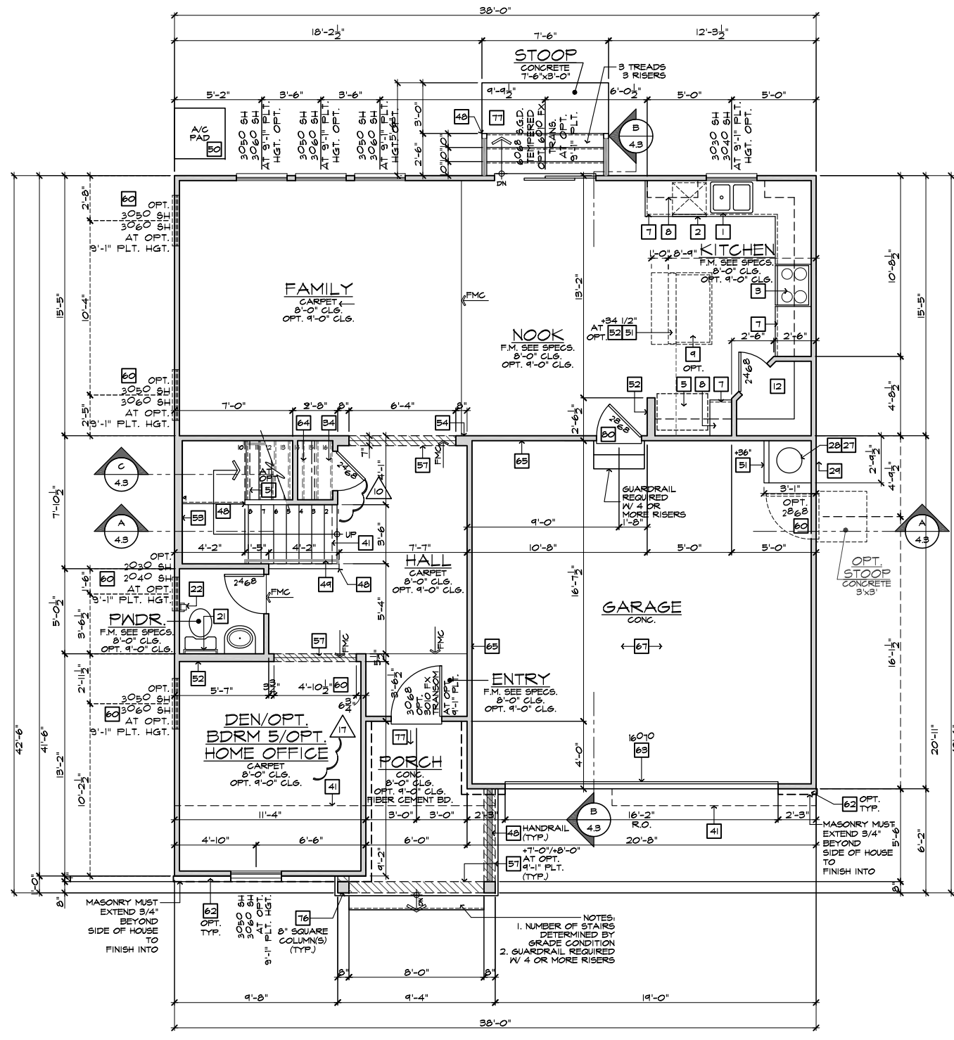
FIRST FLOOR PLAN 'A' W/ CRAWL SPACE SCALE 1/4"=1'-0" (22"X34") - 1/8"=1'-0" (11"X17") AT CRAWLSPACE
