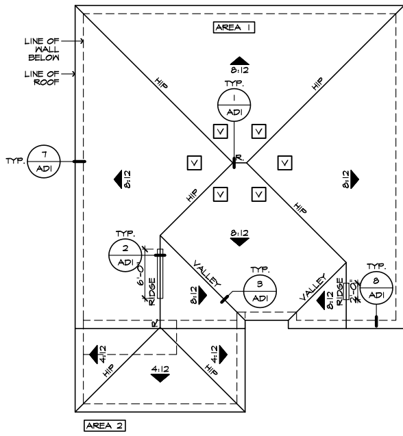
ROOF PLAN 'D' SCALE 1/8"=1'-0" (22'x34') - 1/16"=1'-0" (11'x17')
