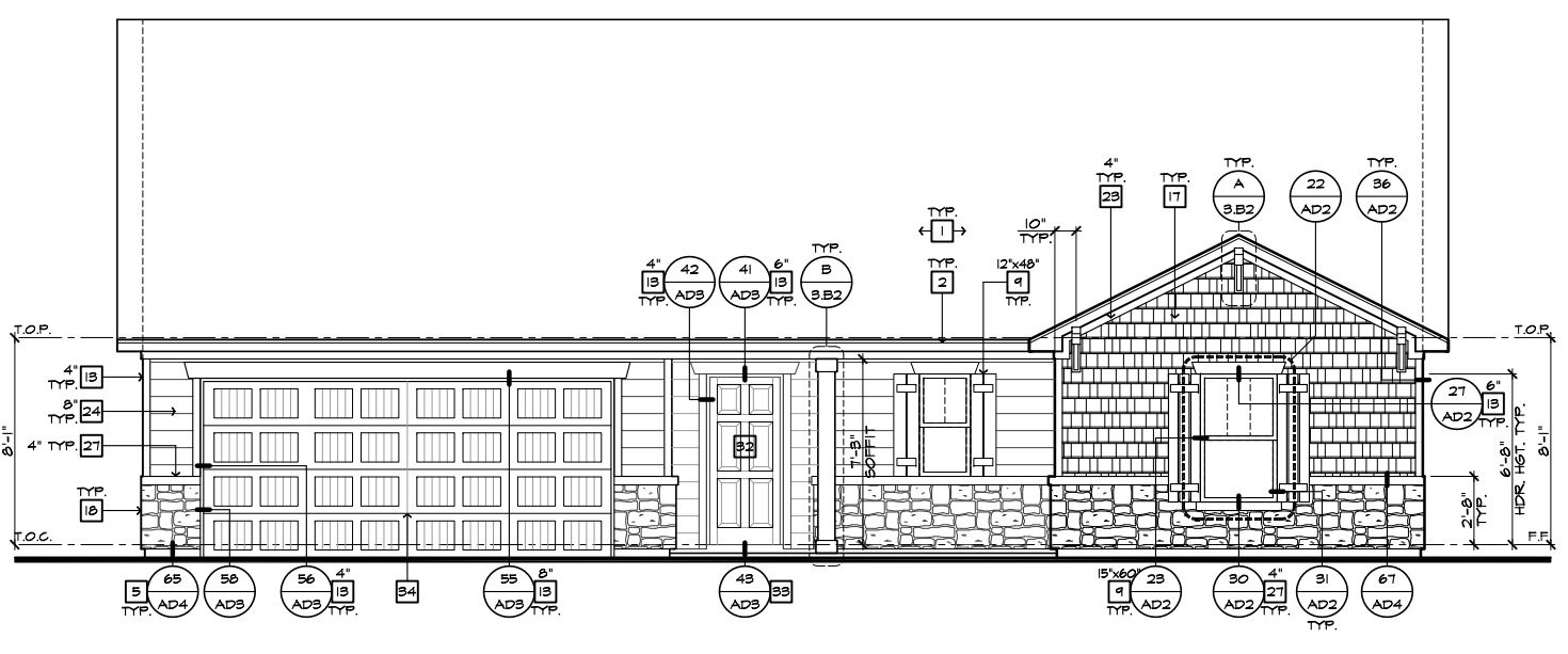
FRONT ELEVATION 'B' W/ STONE OPTION SCALE 1/4"=1'-0" (22'x34") - 1/8"=1'-0" (11'x17")
