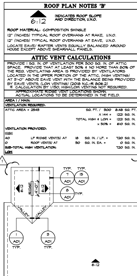
PARTIAL ROOF PLAN
