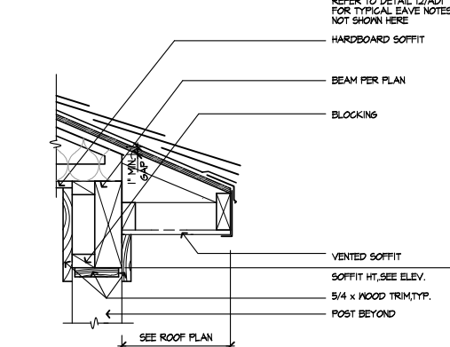
PORCH EAVE
