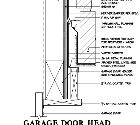
GARAGE DOOR HEAD W/ ARCHED BRICK
