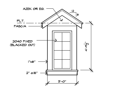
GABLE ROOF DORMER
