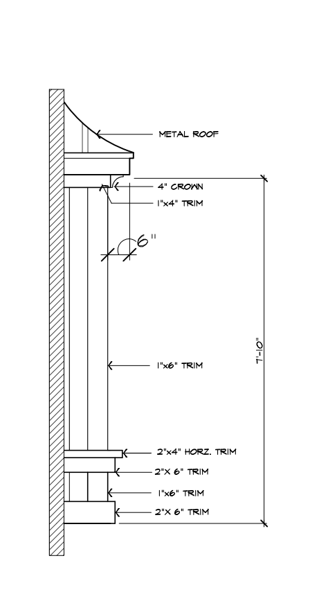
BAY (2)
