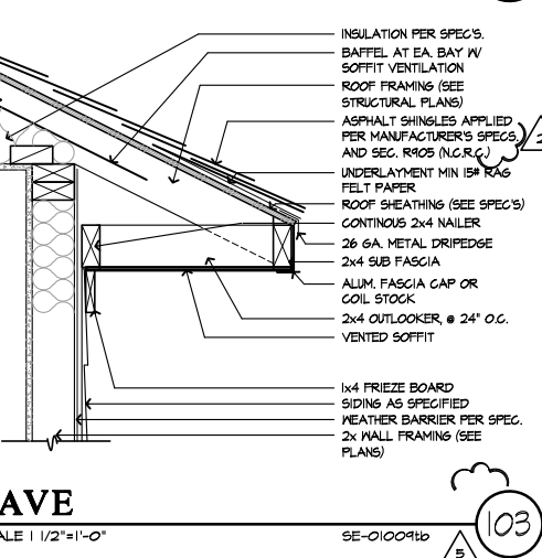
103 EAVE SCALE 1 1/2"=1'-0" SE-010091b
