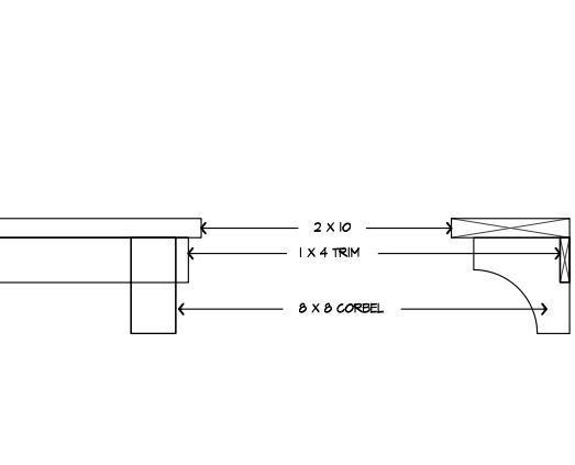
WINDOW LEDGE
