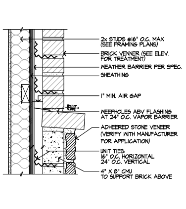
BRICK OVER STONE
