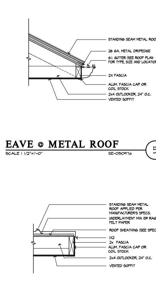
EAVE @ METAL ROOF
