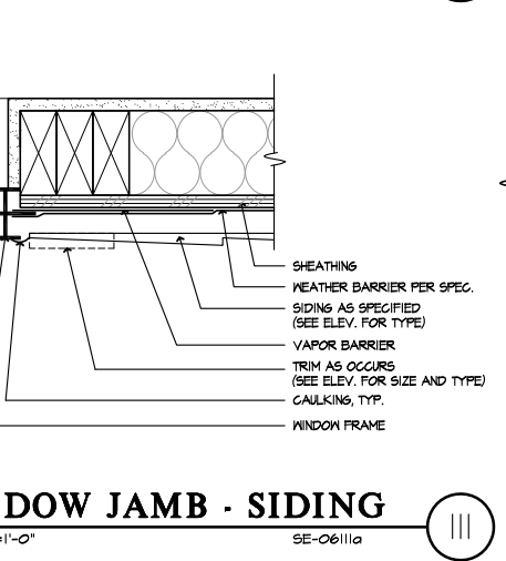
111 WINDOW JAMB - SIDING SCALE 3"=1'-0" SE-06111a
