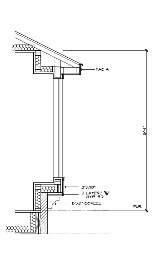
BAY (2)
