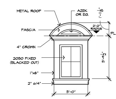
ARCHED ROOF DORMER NOT TO SCALE
