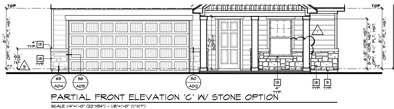
FRONT ELEVATION 'C' SCALE 1/4"=1'-0" (22"x34") - 1/8"=1'-0" (11"x17")
