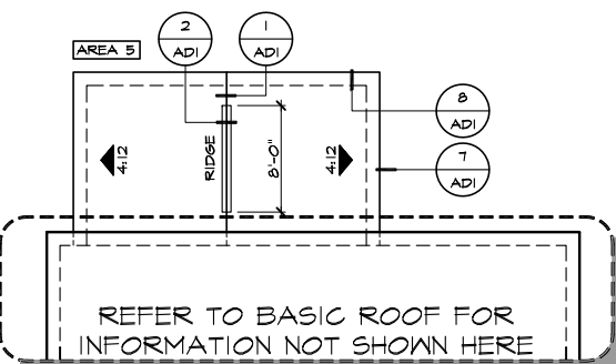
PARTIAL CRAWL SPACE PLAN
