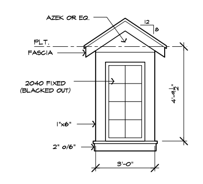
GABLE ROOF DORMER NOT TO SCALE
