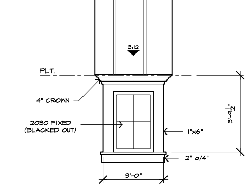
TYP. SHED ROOF DORMER NOT TO SCALE
