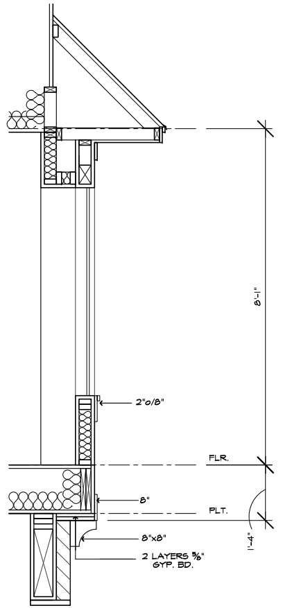
BAY NOT TO SCALE
