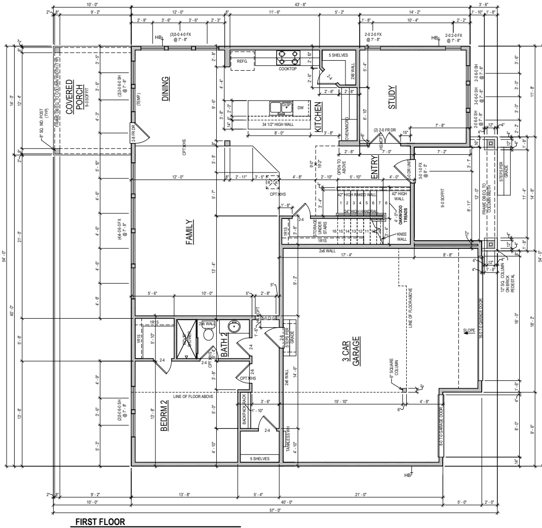
FIRST FLOOR
