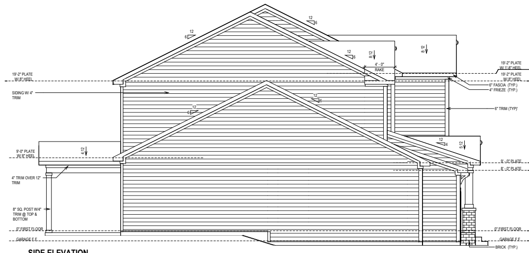
SIDE ELEVATION
