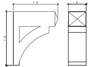
BRACKET DETAIL - BKT15X18X6 SCALE: 1" = 1'-0"
