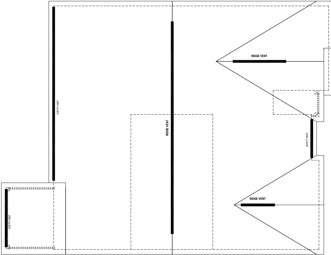
ATTIC VENT CALCULATION
