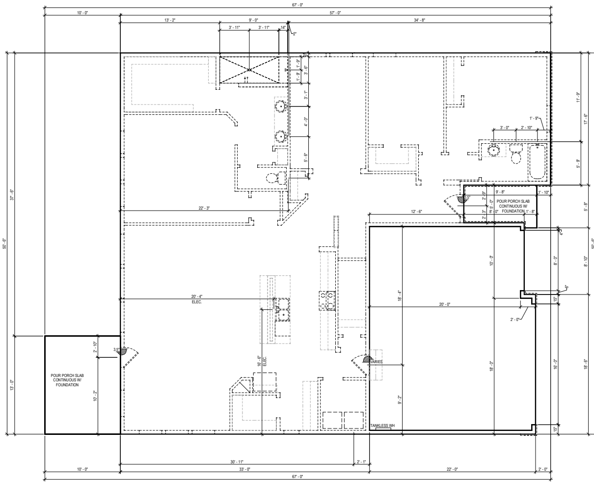
FIRST FLOOR
