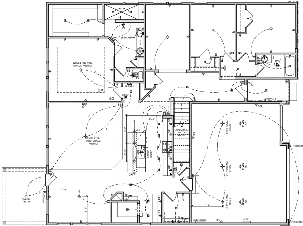
FIRST FLOOR
