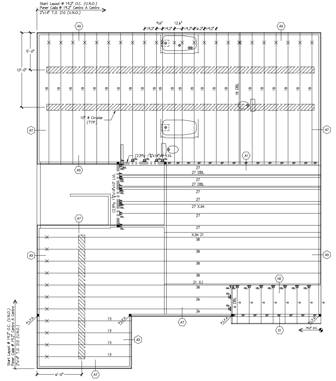
2ND FLOOR I-JOIST PLACEMENT PLAN MATTAMY HOMES - SHENANDOAH
