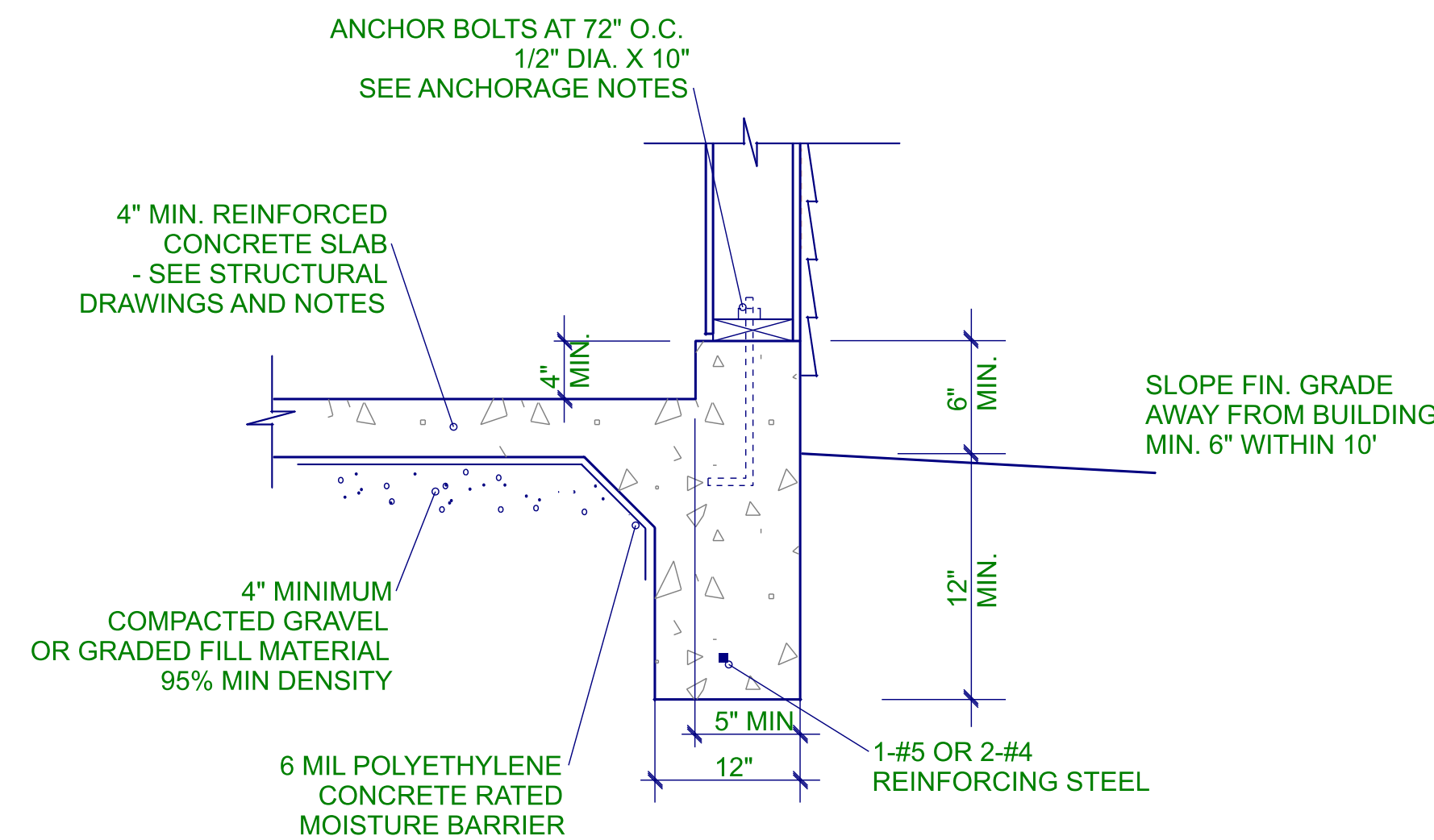
MONOLITHIC SLAB 5\"/>
