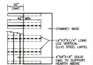
D010 PLAN VIEW OF SUSPENDED HEARTH
