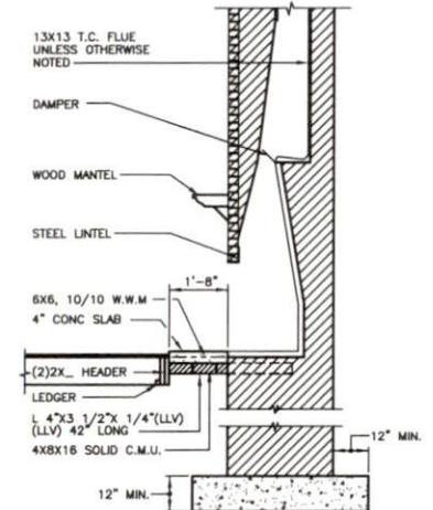
D007 SECT. THRU FIREPLACE ON WOOD FLOOR
