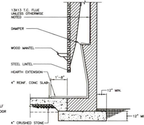
D006 SECT. THRU FIREPLACE ON CONCRETE SLAB
