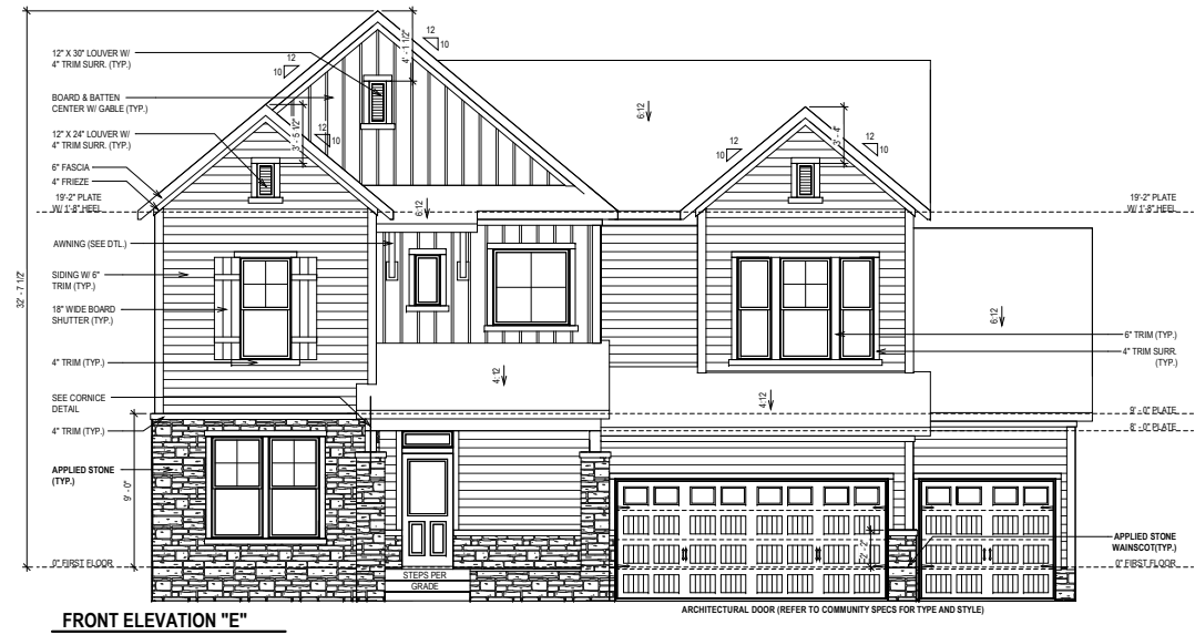
FRONT ELEVATION "E"
