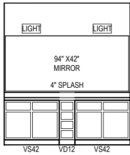
OWNER'S BATH W/ SUPERSHOWER
