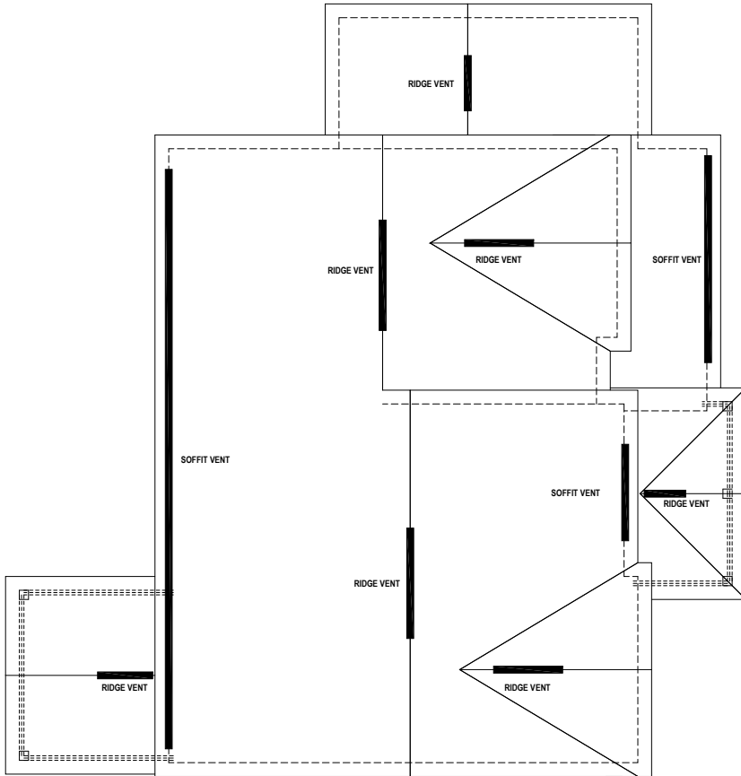
ROOP PLAN CALCS.
