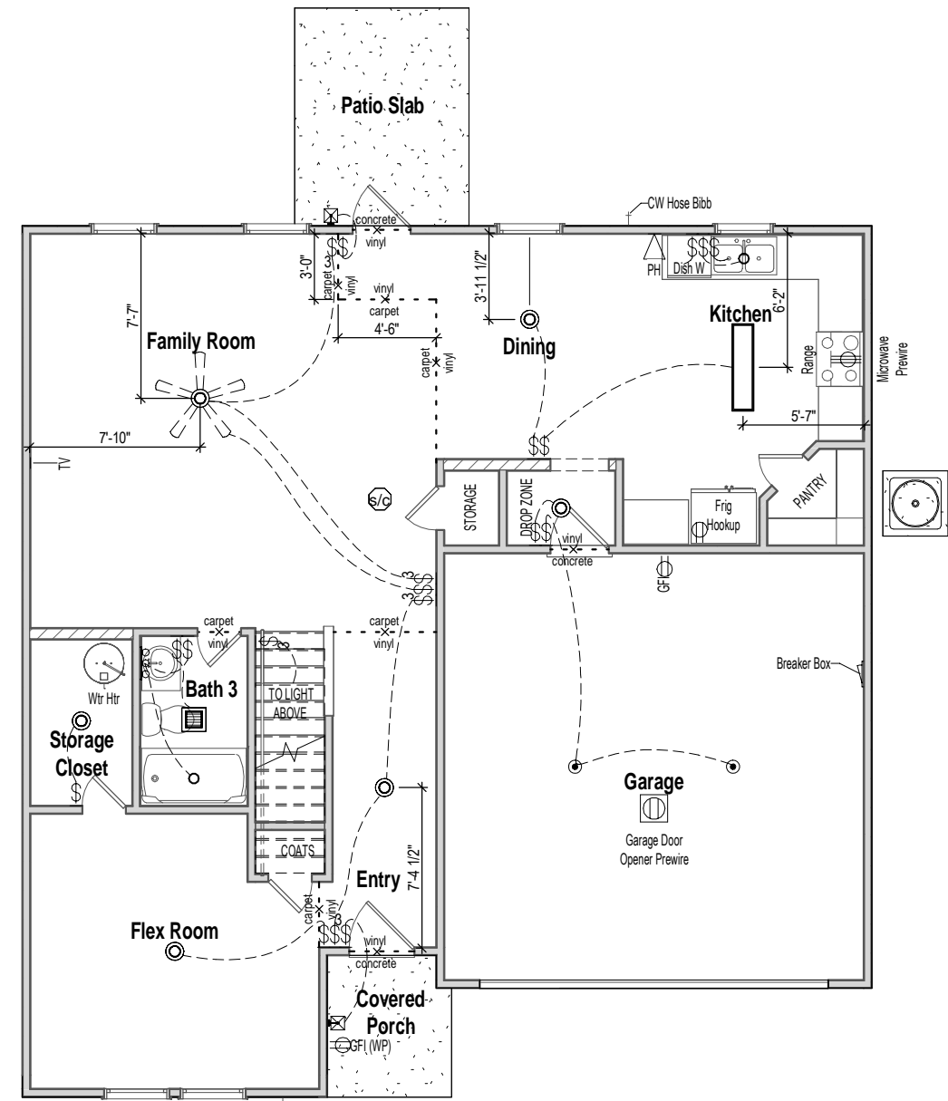
1 1st Floor Electrical - Elev A 1/8" = 1'-0"
