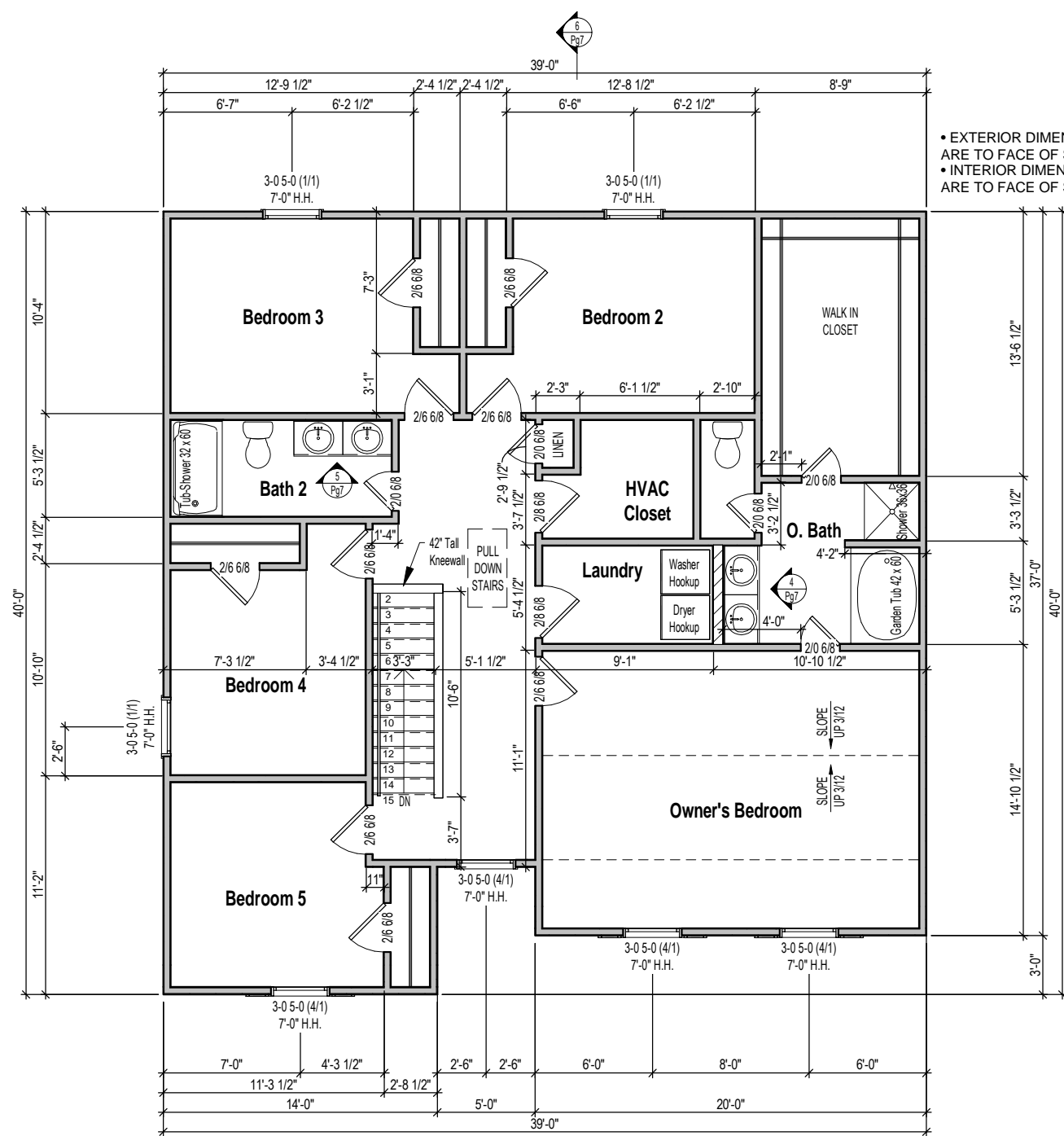
1 2nd Floor Plan - Elev A 1/8" = 1'-0"
