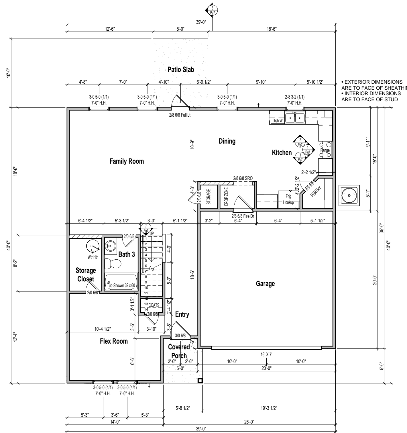
1 1st Floor Plan - Elev A 1/8" = 1'-0"
