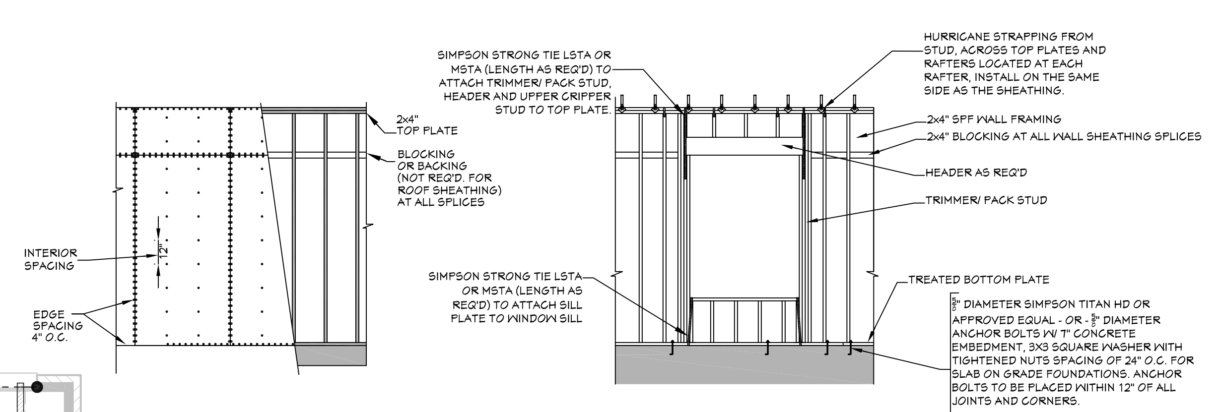
802 WALL/ROOF FASTENING DETAILS SCALE----- 1/4" = 1'-0"
