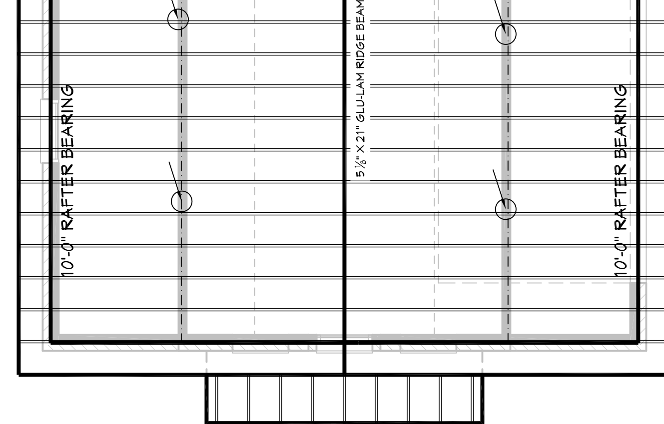
701 ROOF FRAMING SCALE----- 1/4" = 1'-0"
